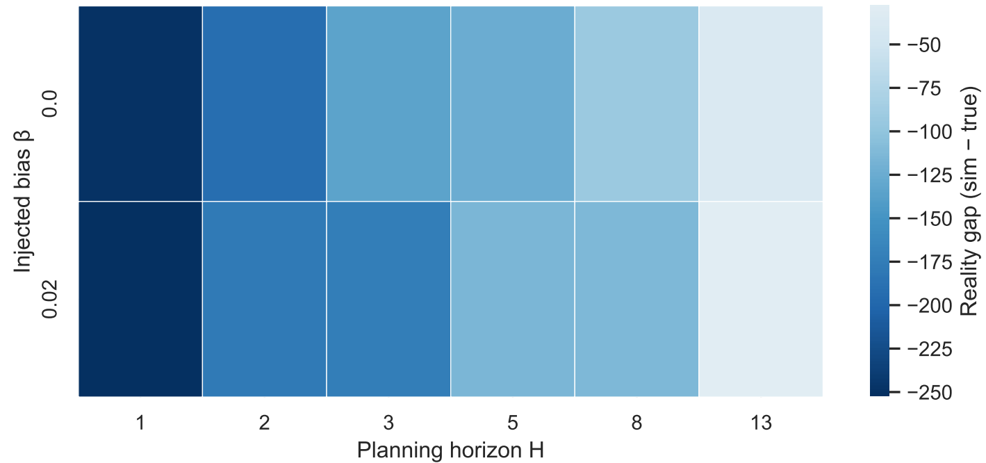
Randomized regime: reality gap heatmap ( \gamma=0.95 )
