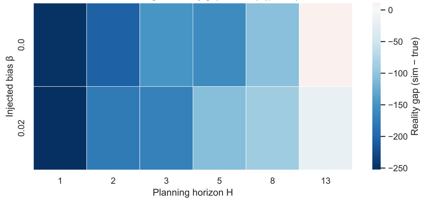
Randomized regime: reality gap heatmap ( \gamma=0.99 )
