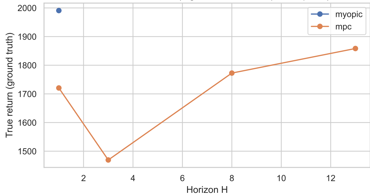
True return vs horizon (regime=confounded, \gamma=0.95 , \beta=0.0 )
