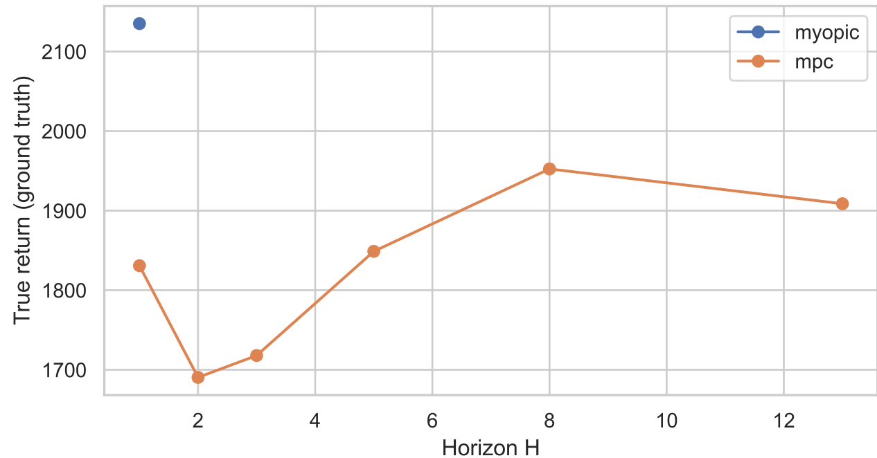
True return vs horizon (regime=randomized, \gamma=0.99 , \beta=0.0 )
