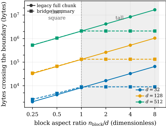
Full local rank: tall blocks compress, flat blocks do not
