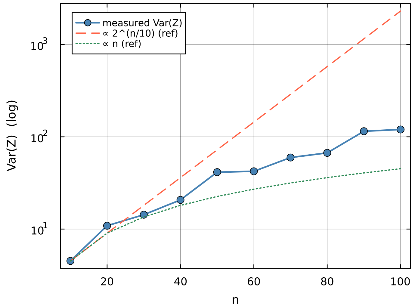
log scale: bounded, not exponential
