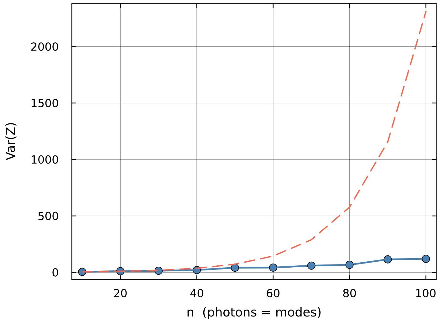
Estimator variance vs system size ( S \approx 0.5 )
