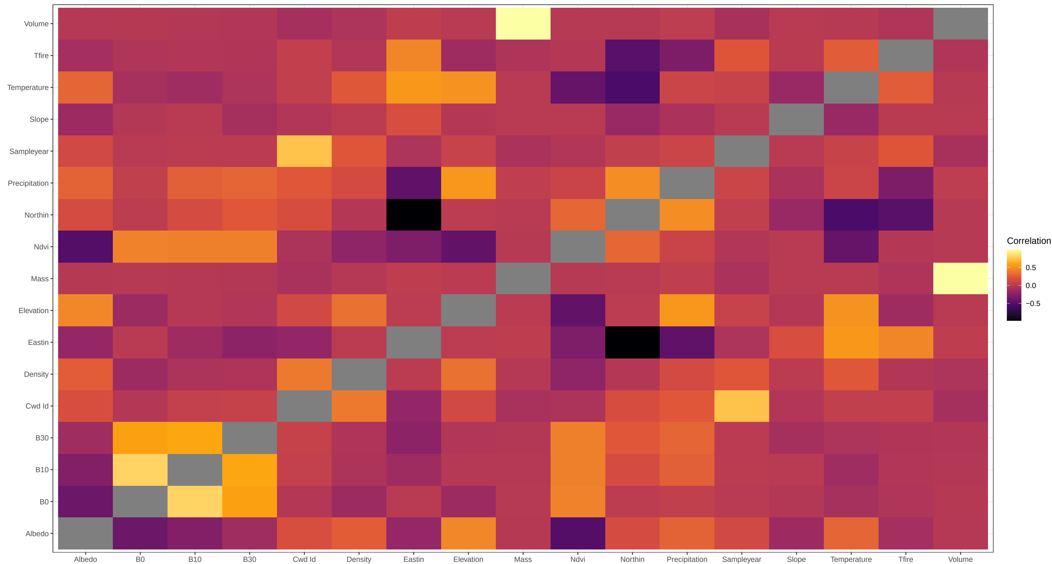
Correlation Matrix of: CWD Biomass Qualitative Variables
