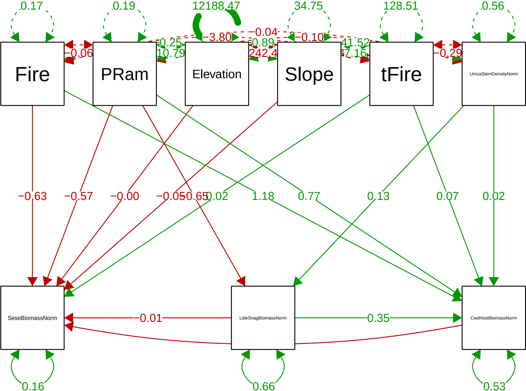
Path analysis quantifying CWD fuels as a mediator for disease driven fire impacts to Redwood biomass
