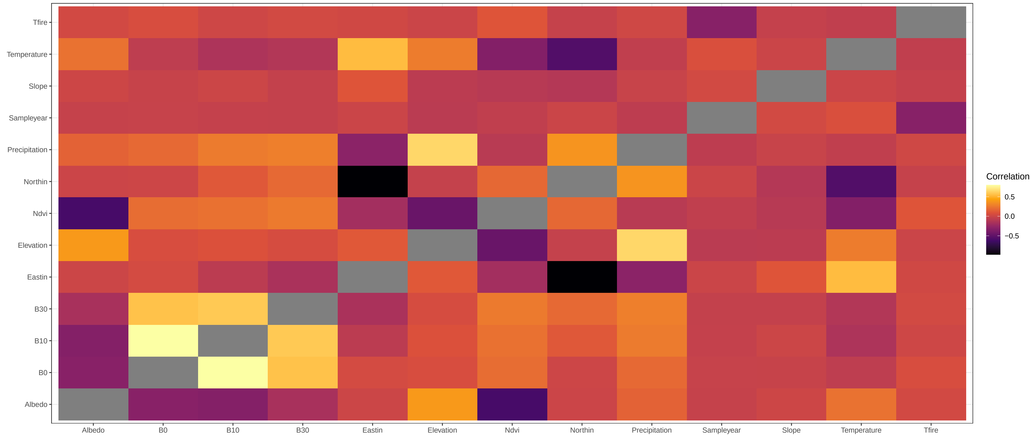
Correlation Matrix of: Plot Qualitative Variables
