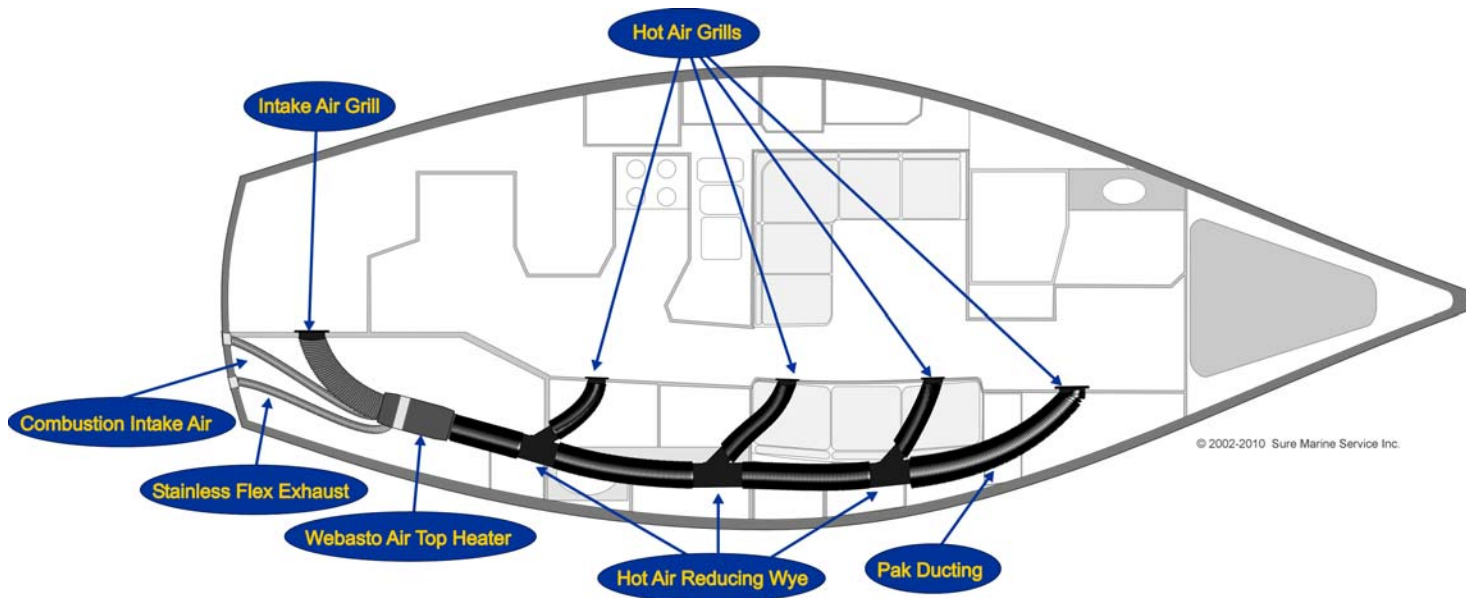
Example of Sailboat Installation of Webasto Air Top 55
