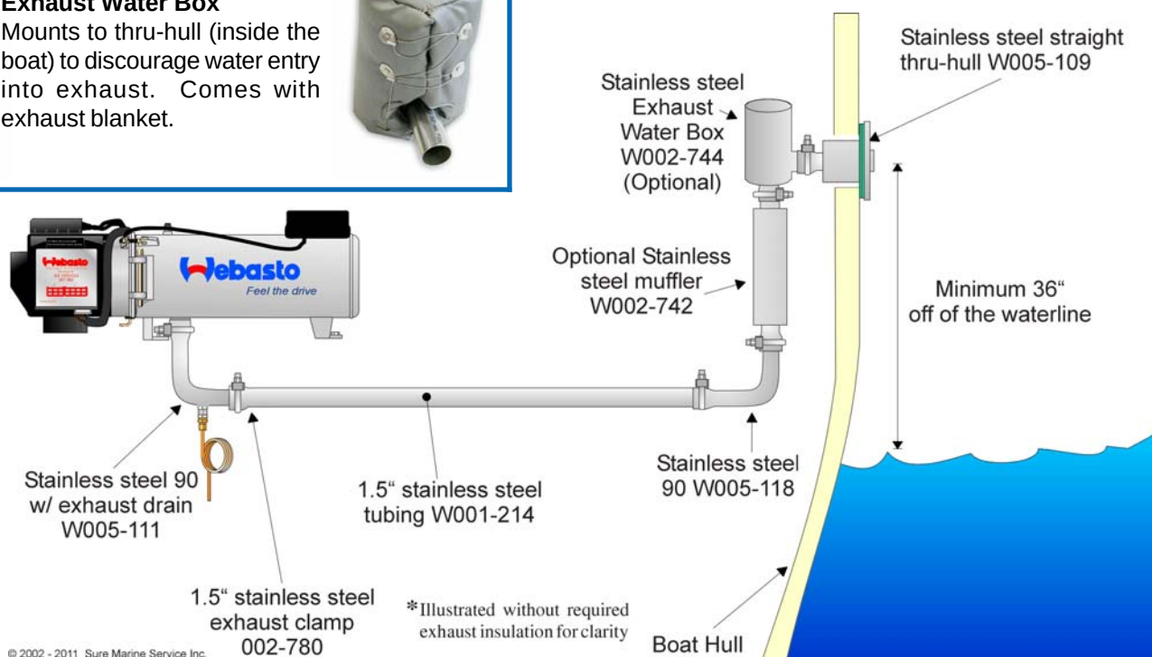
W002-744 1 1/2" Stainless Steel Exhaust Water Box
