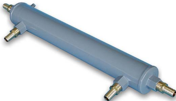
W001-236- \frac{3}{4} " 4" x 24" Heat Exchanger-- \frac{3}{4} " Fittings W001-236-1 \frac{1}{4} " 4" x 24" Heat Exchanger--1 \frac{1}{4} " Fittings
