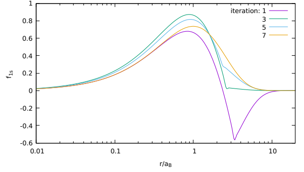
Figure 1: Hydrogen 1s orbital [ f(r) ], as calculated at the first through 7th iteration. For this example, the initial energy guess was -0.3 au, and converged to -0.500006566.. au to parts in 10^{-16} in 12 iterations.
