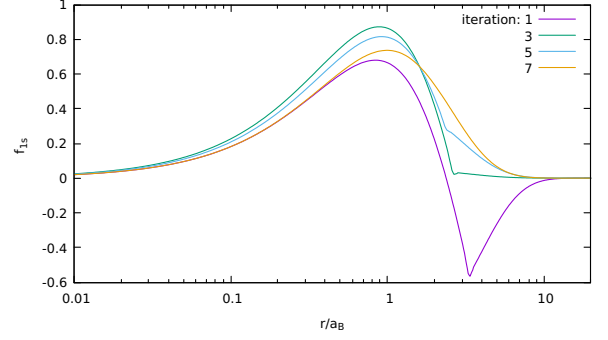
Figure 1: Hydrogen 1s orbital [ f(r) ], as calculated at the first though 7th iteration. For this example, the initial energy guess was -0.3 au, and converged to -0.500006566.. au to parts in 10^{-16} in 12 iterations.
