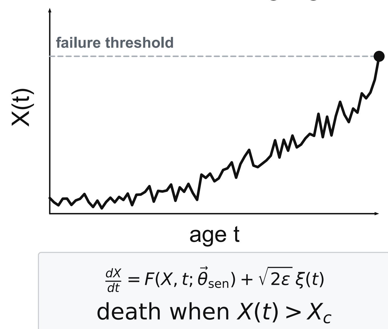
a Stochastic threshold-crossing view of aging
