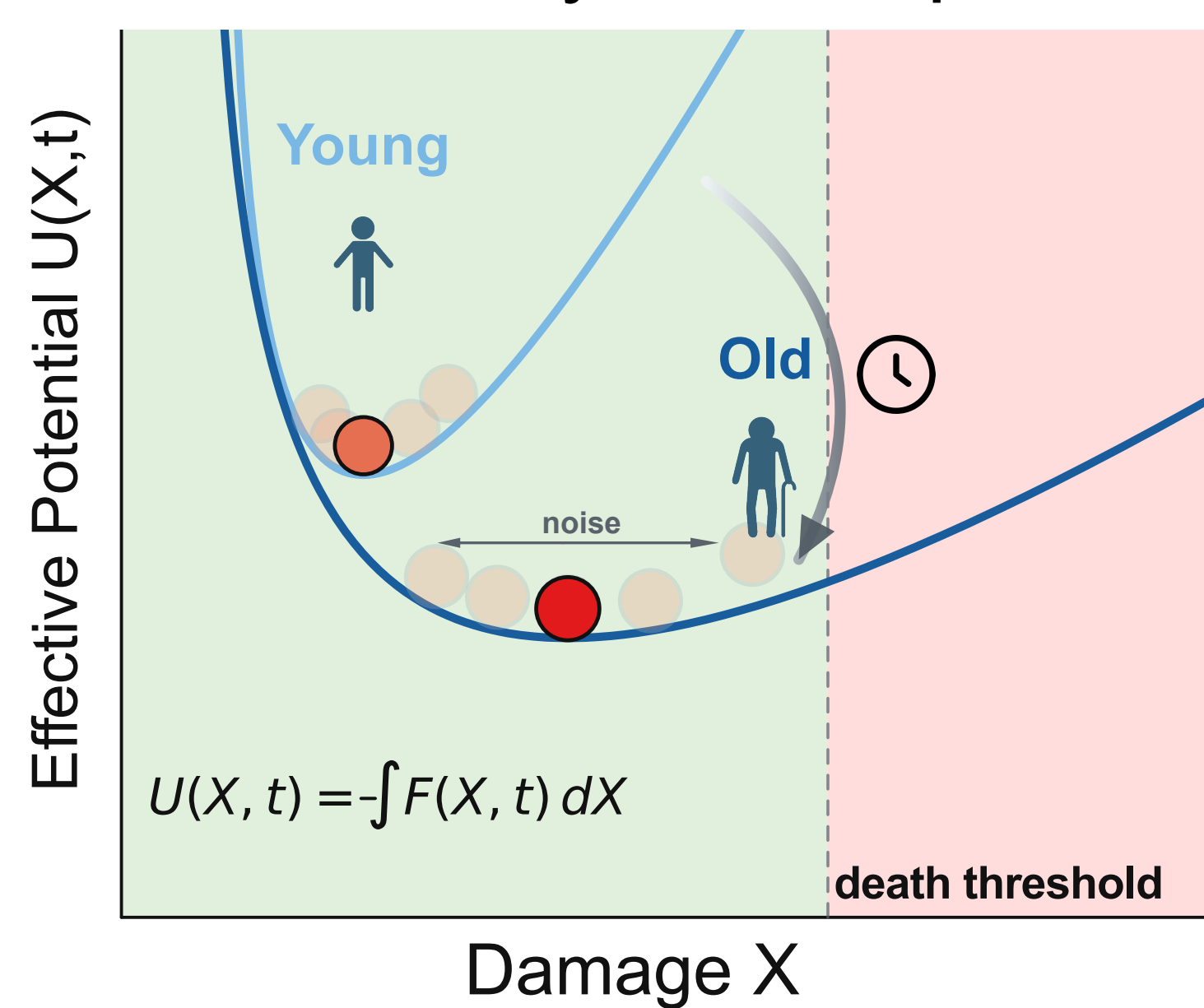
b Dynamics within a flattening stability landscape
