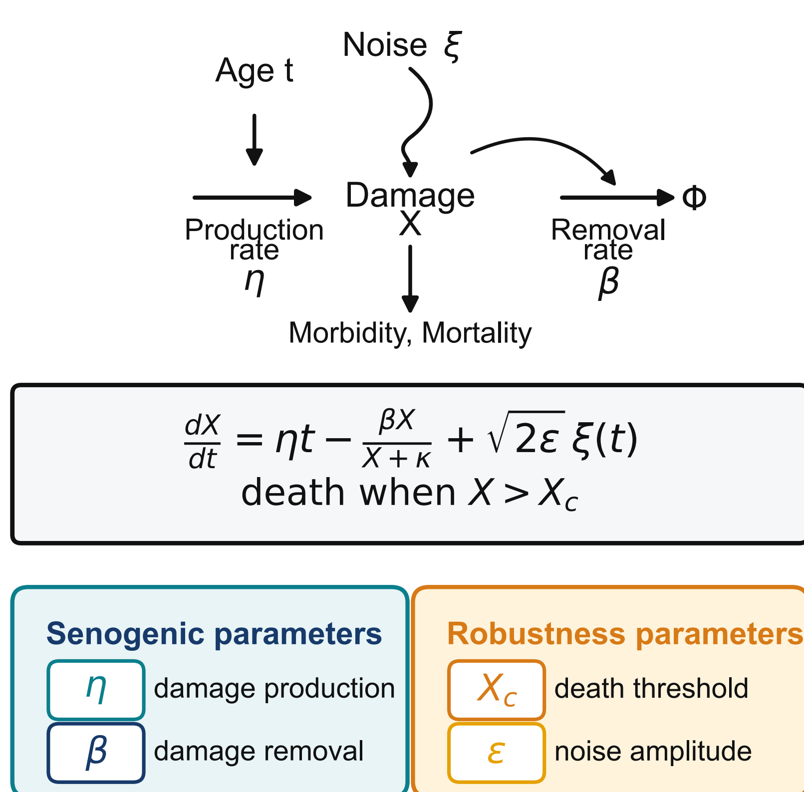
e Saturating-removal model
