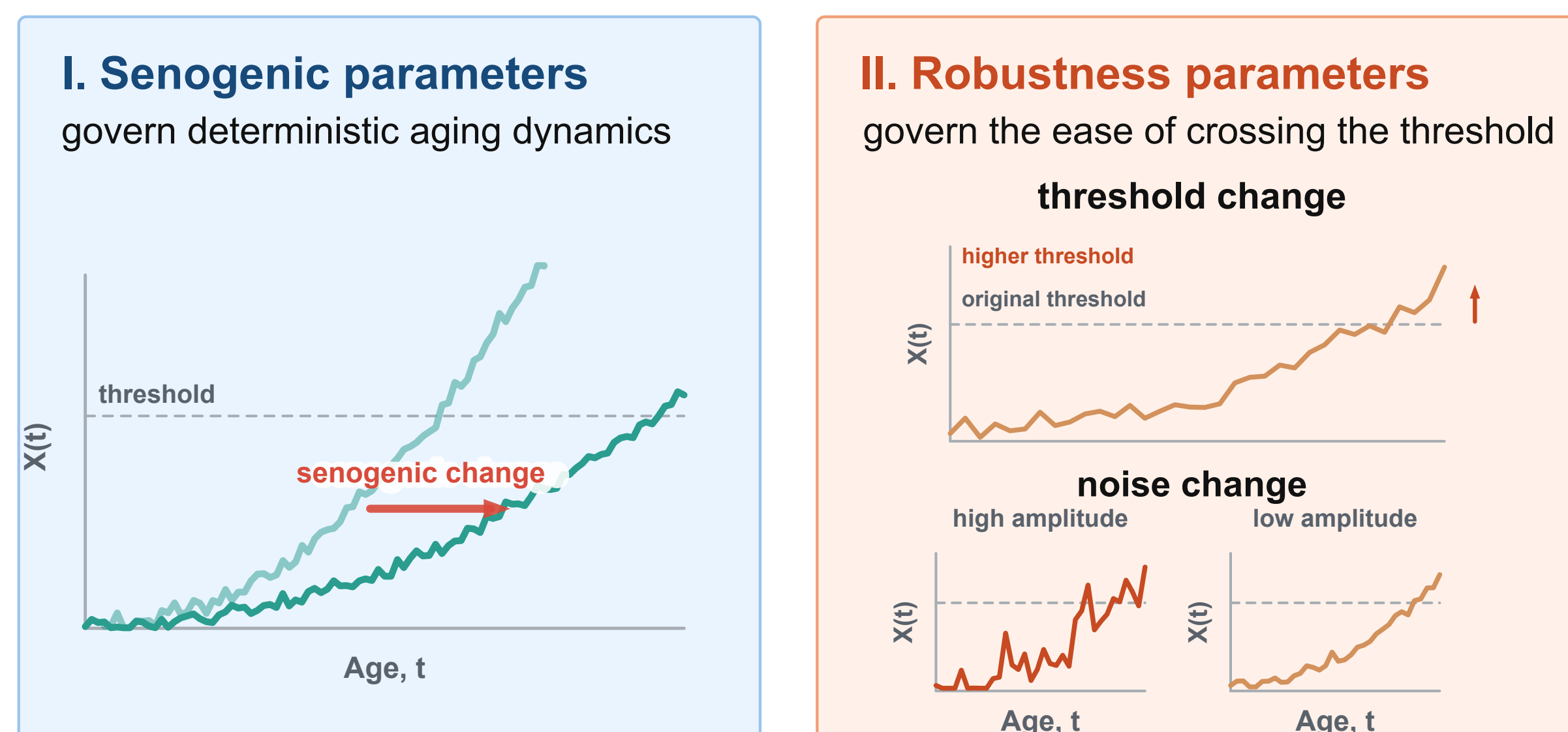
c Two classes of parameters
