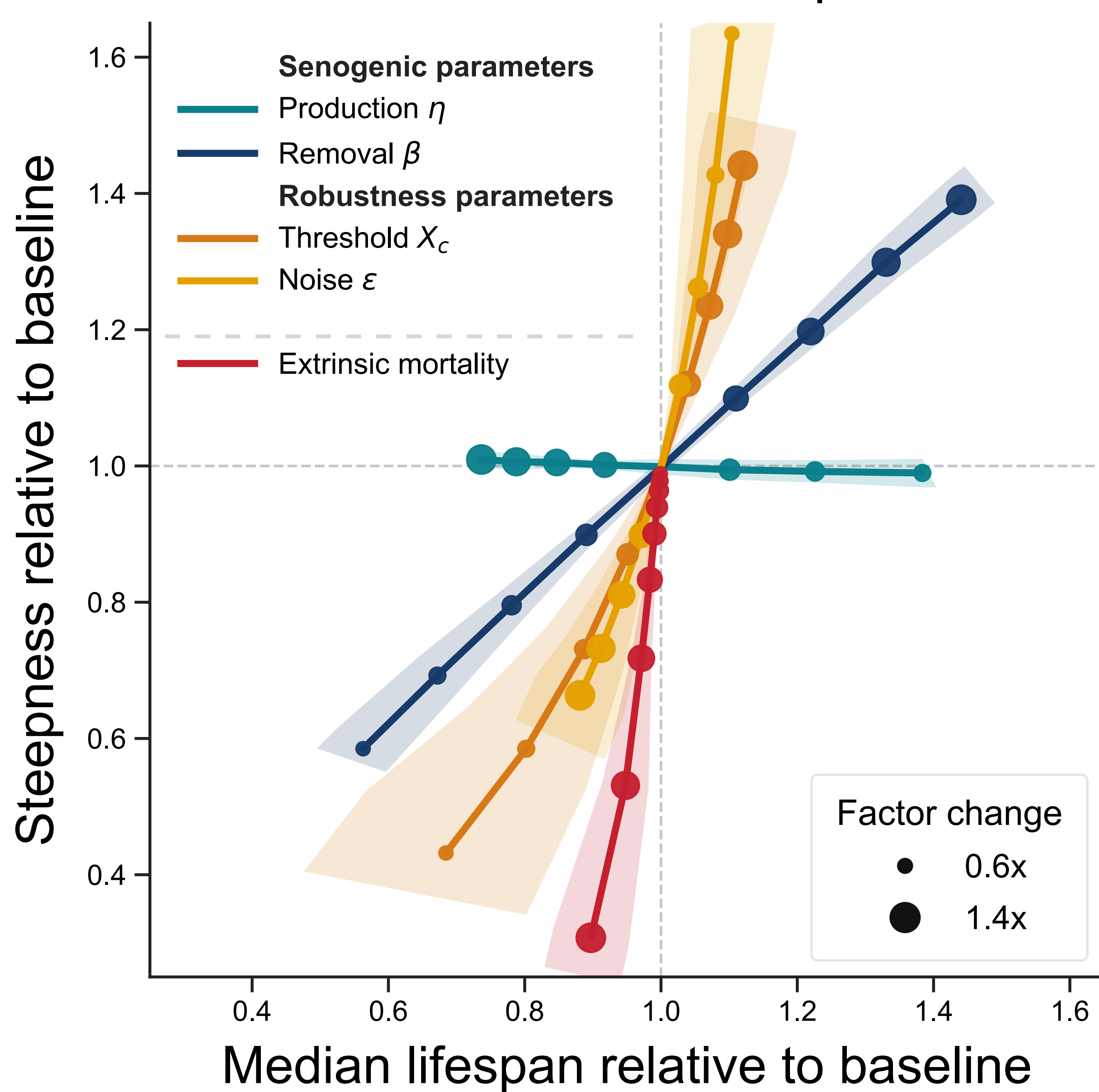
g Parameter change effect on survival curve shape
