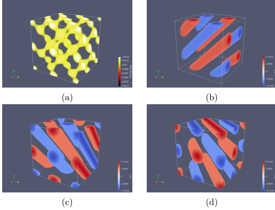
Figure 3.1: Isosurfaces of vorticity \omega = \nabla \times \boldsymbol{\eta}_{TGV} (a) magnitude |\omega(\mathbf{x})| , and components (b) |\omega_1| , (c) |\omega_2| , and (d) |\omega_3| .
