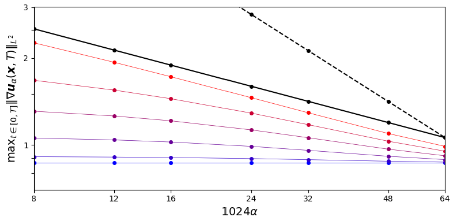
Figure 5.5: Solution of the Euler-Voigt system for T = 5 starting from \boldsymbol{\eta}_{TGV} . Log-log plot of \max_{t \in [0, T]} \|\nabla \mathbf{u}_\alpha(t)\|_{L^2} vs \alpha at t = 0 (blue) to t = 5 (red), Steepest slope p = -0.417 (black), slope of p = -1 (dotted black)
