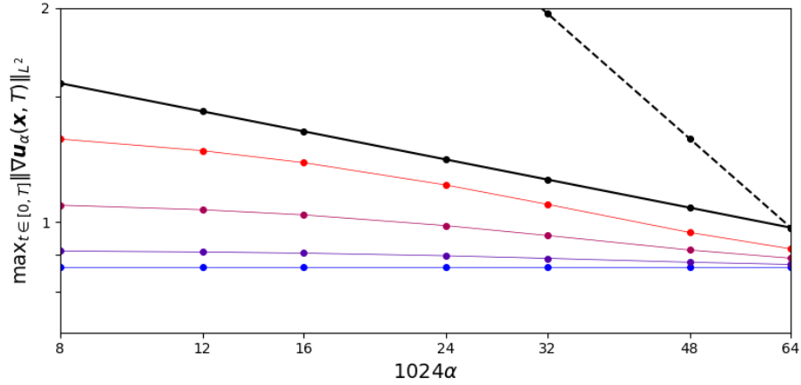
Figure 5.3: Solution of the Euler-Voigt system for T = 3 starting from \boldsymbol{\eta}_{TGV} . Log-log plot of \max_{t \in [0, T]} \|\nabla \mathbf{u}_\alpha(t)\|_{L^2} vs \alpha at t = 0 (blue) to t = 3 (red), Steepest slope p = -0.225 (black), slope of p = -1 (dotted black)
