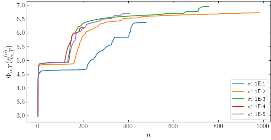
Figure 4.6: \Phi_{\alpha,T}(\eta_{\alpha,T}^{(n)}) vs iteration number n for \alpha = 16/1024 , T = 5 , and different indicated values of \sigma .
