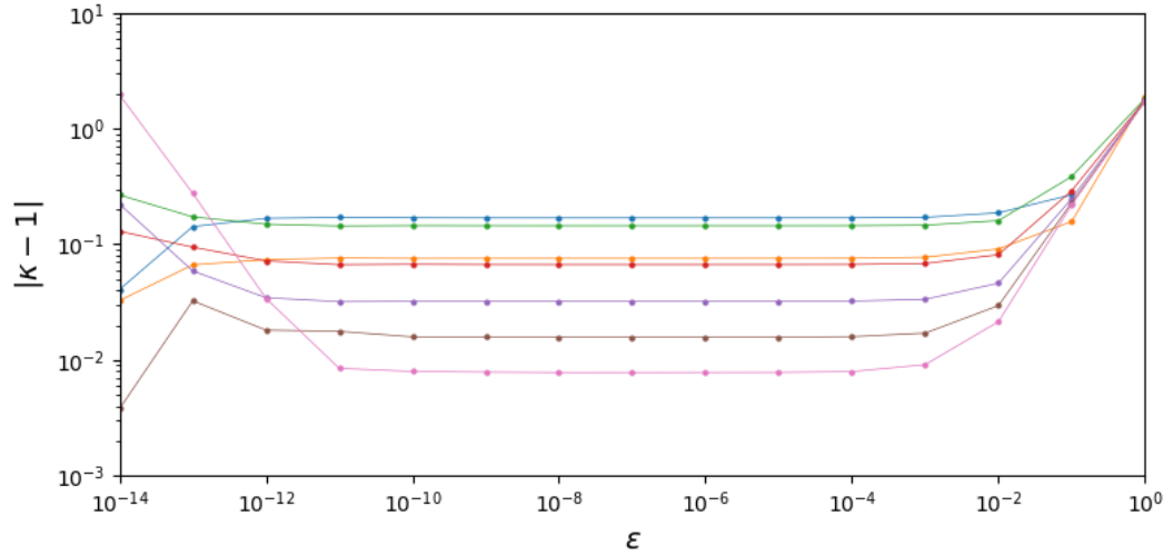
Figure 4.4: Dependence of \kappa(\epsilon) on \epsilon for \alpha = 8/1024 .
