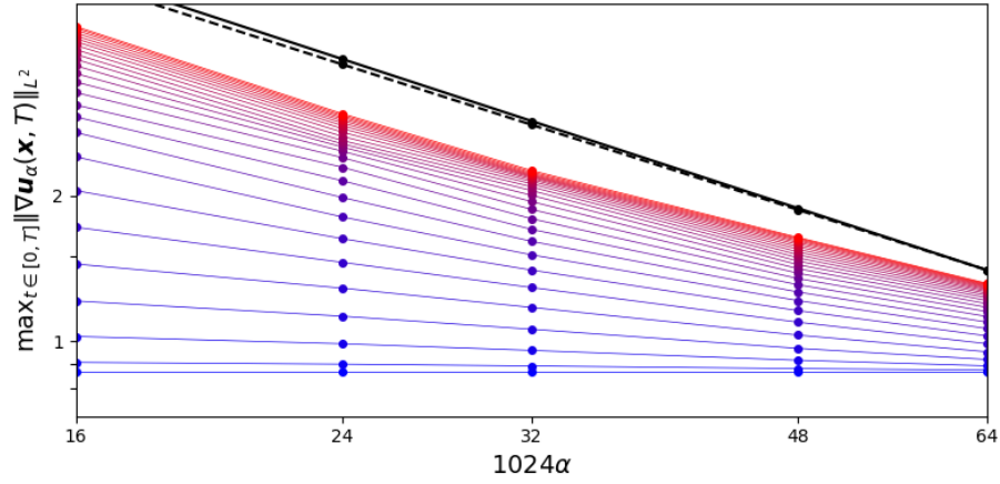
Figure 5.7: TGV for T = 25 . Log-log plot of \max_{t \in [0, T]} \|\nabla \mathbf{u}_\alpha(t)\|_{L^2} vs \alpha at t = 0 (blue) to t = 25 (red), Steepest slope p = (black), slope of p = -1 (dotted black)
