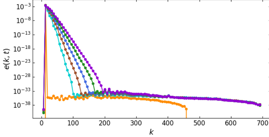
Figure 4.2: e(k, t) vs. k starting from \boldsymbol{\eta}_{TGV} for \alpha = 64/1024 and N = 128^3 at t = 0 (orange), t = 1 (cyan), t = 2 (brown), t = 3 (blue), t = 4 (green), t = 5 (purple).
