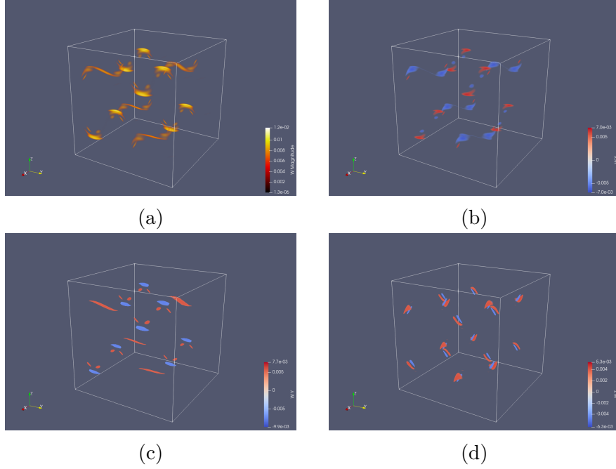
Figure 5.2: Isosurfaces of vorticity \omega = \nabla \times \mathbf{u}_\alpha(T = 5; \boldsymbol{\eta}_{TGV}) . (a) magnitude |\omega(\mathbf{x})| , and components (b) |\omega_1| , (c) |\omega_2| , and (d) |\omega_3| .
