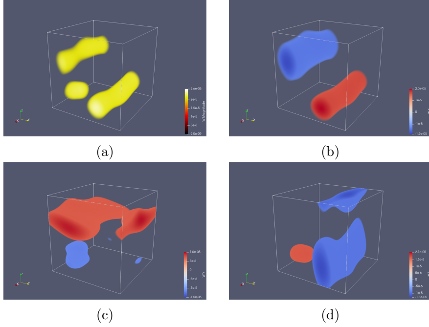
Figure 3.2: Isosurfaces of vorticity \omega = \nabla \times \boldsymbol{\eta}_S (a) magnitude |\omega(\mathbf{x})| , and components (b) |\omega_1| , (c) |\omega_2| , and (d) |\omega_3| .
