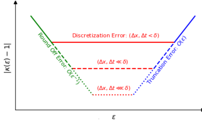
Figure 4.3: Schematic illustration of the log-log dependence of \kappa(\epsilon) on \epsilon , cf. (4.60).
