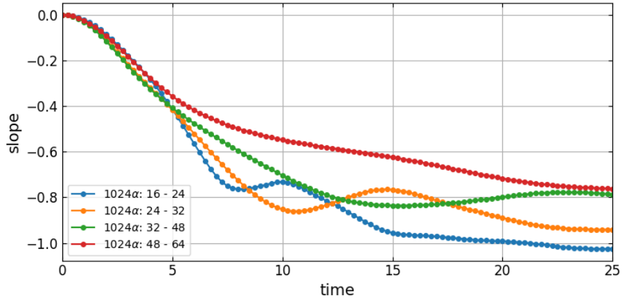
Figure 5.8: TGV for T = 25 . Plot of the slope of (\max_{t \in [0, T]} \|\nabla \mathbf{u}_\alpha(t)\|_{L^2} \text{ vs } \alpha) vs time at each \alpha .
