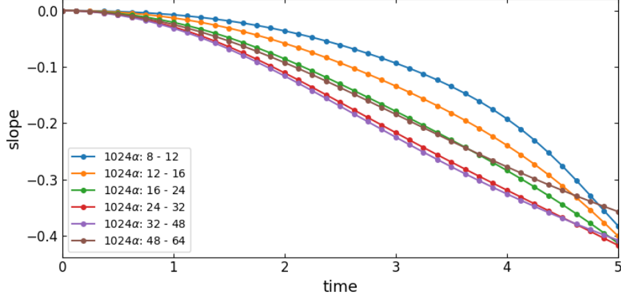
Figure 5.6: Solution of the Euler-Voigt system for T = 5 starting from \boldsymbol{\eta}_{TGV} . Plot of the slope of (\max_{t \in [0, T']} \|\nabla \mathbf{u}_\alpha(t)\|_{L^2} \text{ vs } \alpha) vs time at each \alpha .
