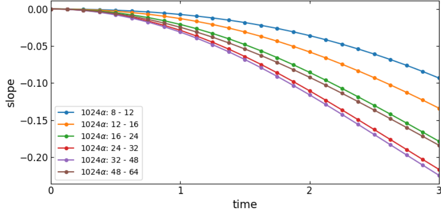
Figure 5.4: Solution of the Euler-Voigt system for T = 3 starting from \boldsymbol{\eta}_{TGV} . Plot of the slope of (\max_{t \in [0, T]} \|\nabla \mathbf{u}_\alpha(t)\|_{L^2}) vs \alpha vs time for each \alpha .
