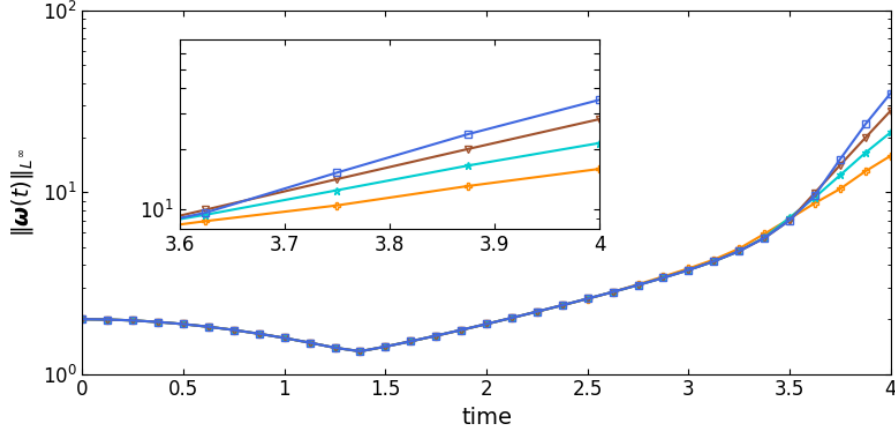
Figure 2.1: Maximum of vorticity \|\boldsymbol{\omega}(t)\|_{L^\infty} . Results from runs performed at different resolutions are displayed together: 128^3 (orange plus), 256^3 (cyan star), 512^3 (brown triangles), 1024^3 (blue squares).
