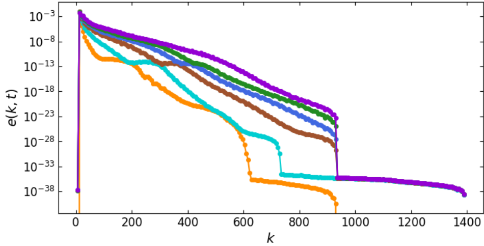
Figure 4.1: e(k, t) vs. k starting from \boldsymbol{\eta}_S for \alpha = 8/1024 and N = 256^3 at t = 0 (orange), t = 1 (cyan), t = 2 (brown), t = 3 (blue), t = 4 (green), t = 5 (purple).
