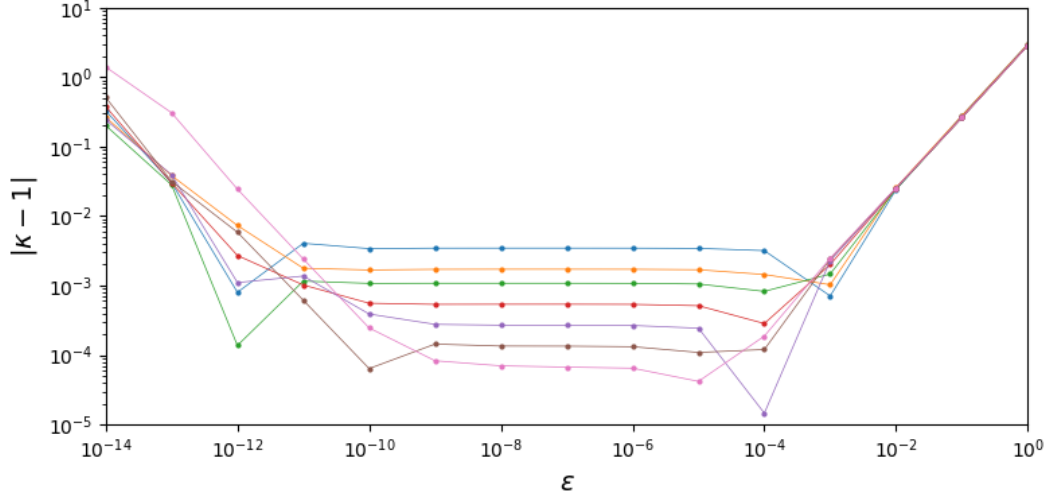
Figure 4.5: Dependence of \kappa(\epsilon) on \epsilon for \alpha = 64/1024 .
