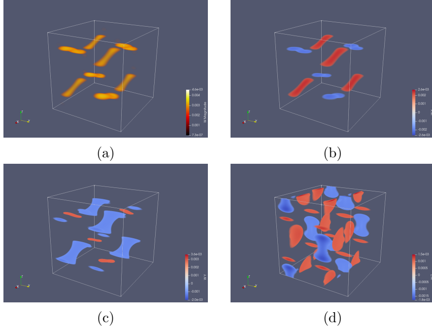
Figure 5.1: Isosurfaces of vorticity \omega = \nabla \times \mathbf{u}_\alpha(T = 3; \boldsymbol{\eta}_{TGV}) . (a) magnitude |\omega(\mathbf{x})| , and components (b) |\omega_1| , (c) |\omega_2| , and (d) |\omega_3| .
