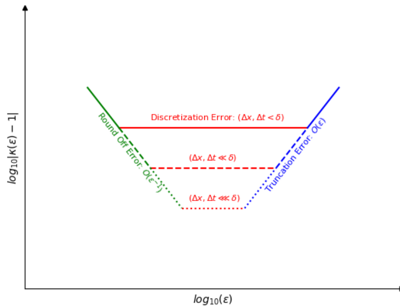
Figure 1: Plot showing the expected \kappa behaviour for different spatial and temporal resolution where \delta represents a small arbitrary constant.
