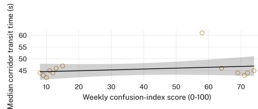
Weekly confusion-index score against median transit time, 14 weeks to 22 June 2026; the two track weakly ( r = 0.23 , n = 14 , p = 0.42 ).
