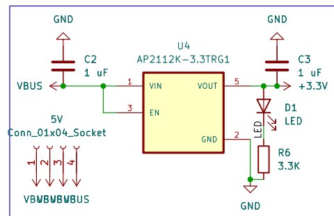
Linear Voltage Regulator to step down voltage from 5V to 3.3V
