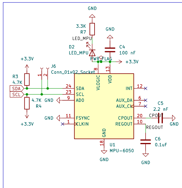
Accelerometer and Gyroscope Sensor
