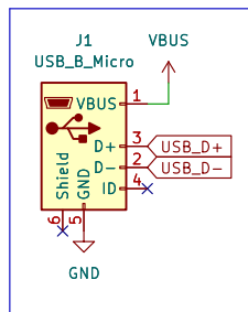
USB Circuitry
