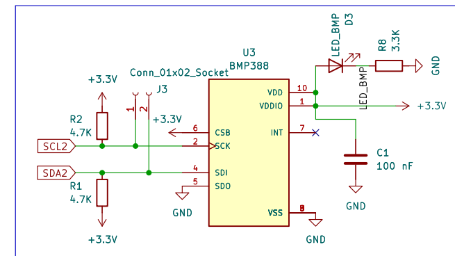
SDO is pulled to ground in order to set address to 1110110
