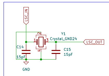
Crystal Circuitry at ~32 kHz
