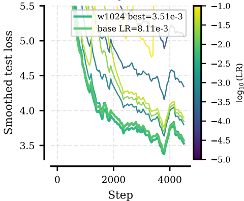
w1024 — test trajectories (12 LRs)
