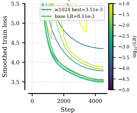
w1024 — train trajectories (12 LRs)
