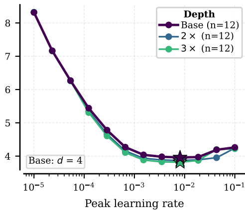
depth scan
