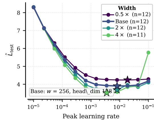
width scan
