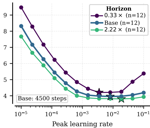
training-horizon scan
