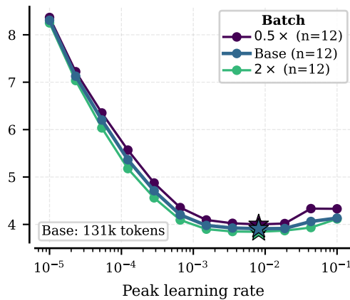
batch-size scan
