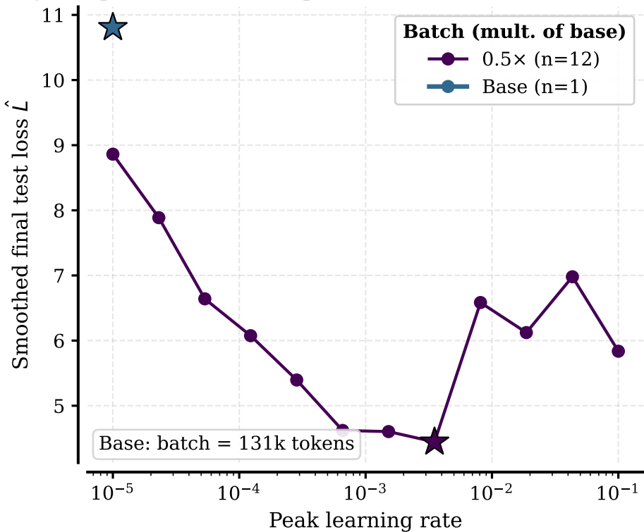
μCompletedP-KL-Shampoo HP transfer — batch-size scan
