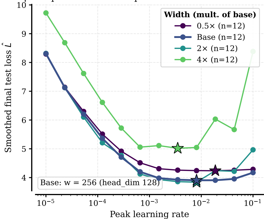
μCompletedP-KL-Shampoo HP transfer — width scan
