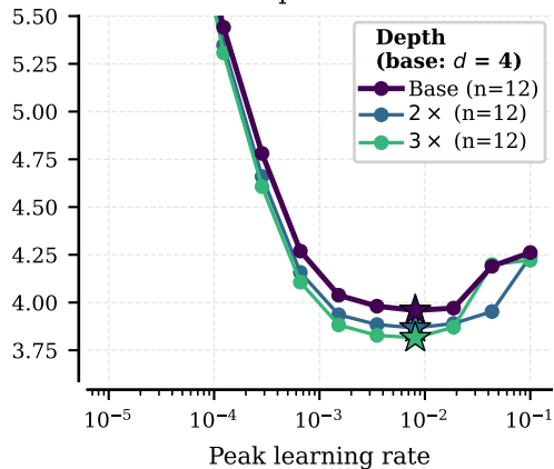
depth scan
