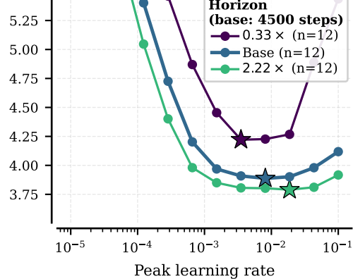
training-horizon scan
