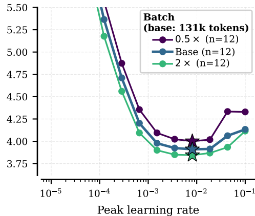
batch-size scan
