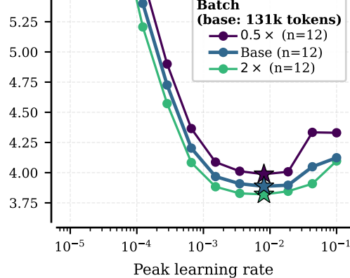
batch-size scan
