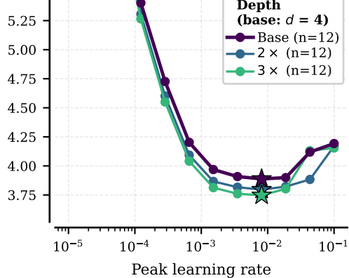
depth scan
