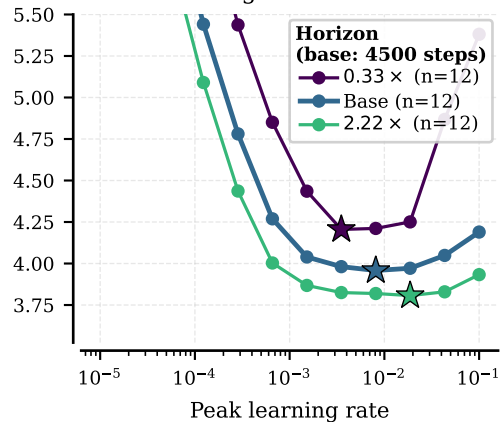
training-horizon scan
