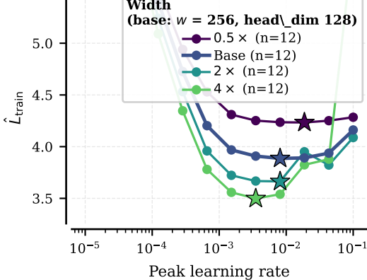
width scan
