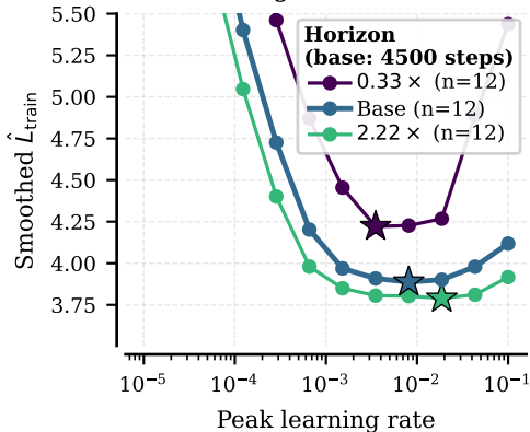
training-horizon scan
