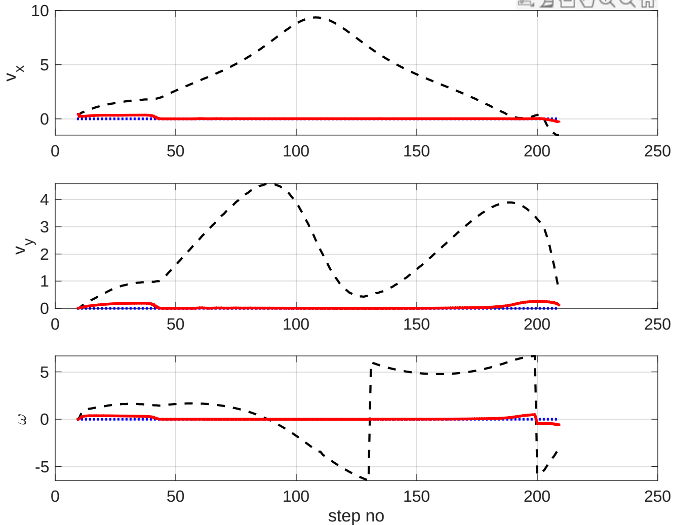
Nominal, Backup, and Filtered Control Inputs
