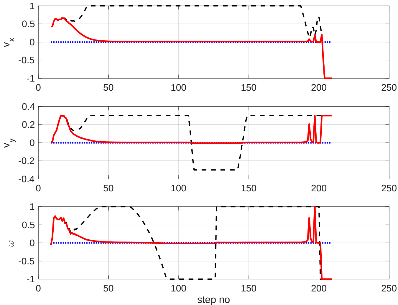
Nominal, Backup, and Filtered Control Inputs
