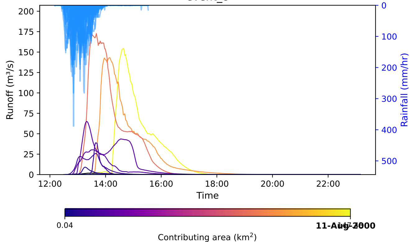
event_8
