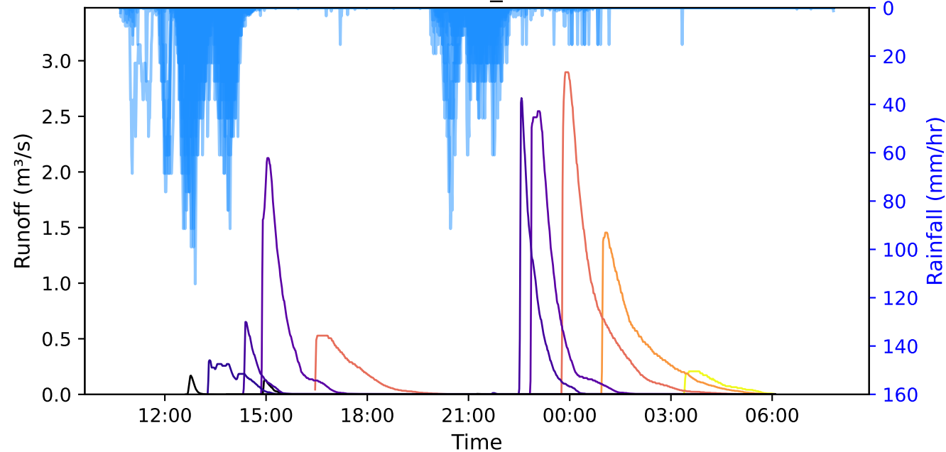
event_45
