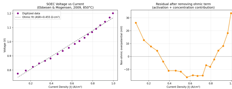
Loss separation
