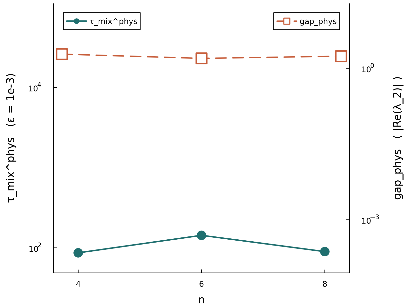
DISORDERED ( \beta_{\text{phys}} = 0.25 )
