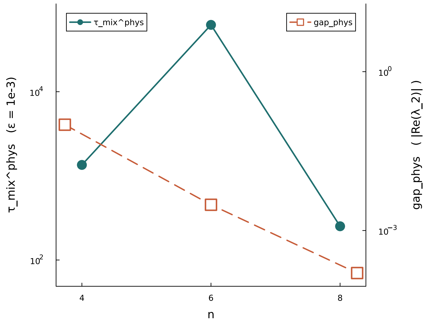
ORDERED ( \beta_{\text{phys}} = 2.0 )
