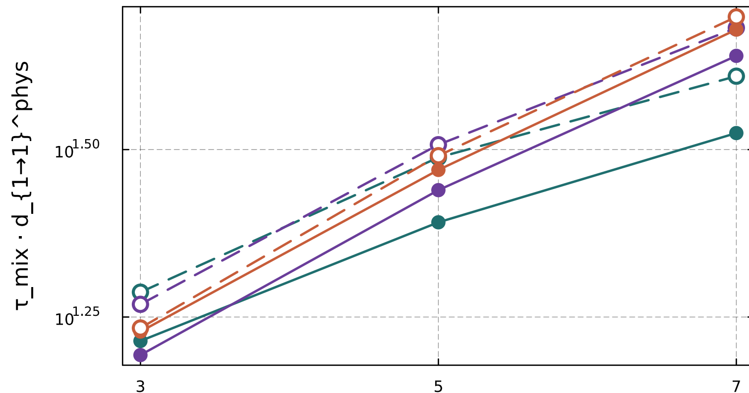
odd-n (d {1→1}-rescaled)
