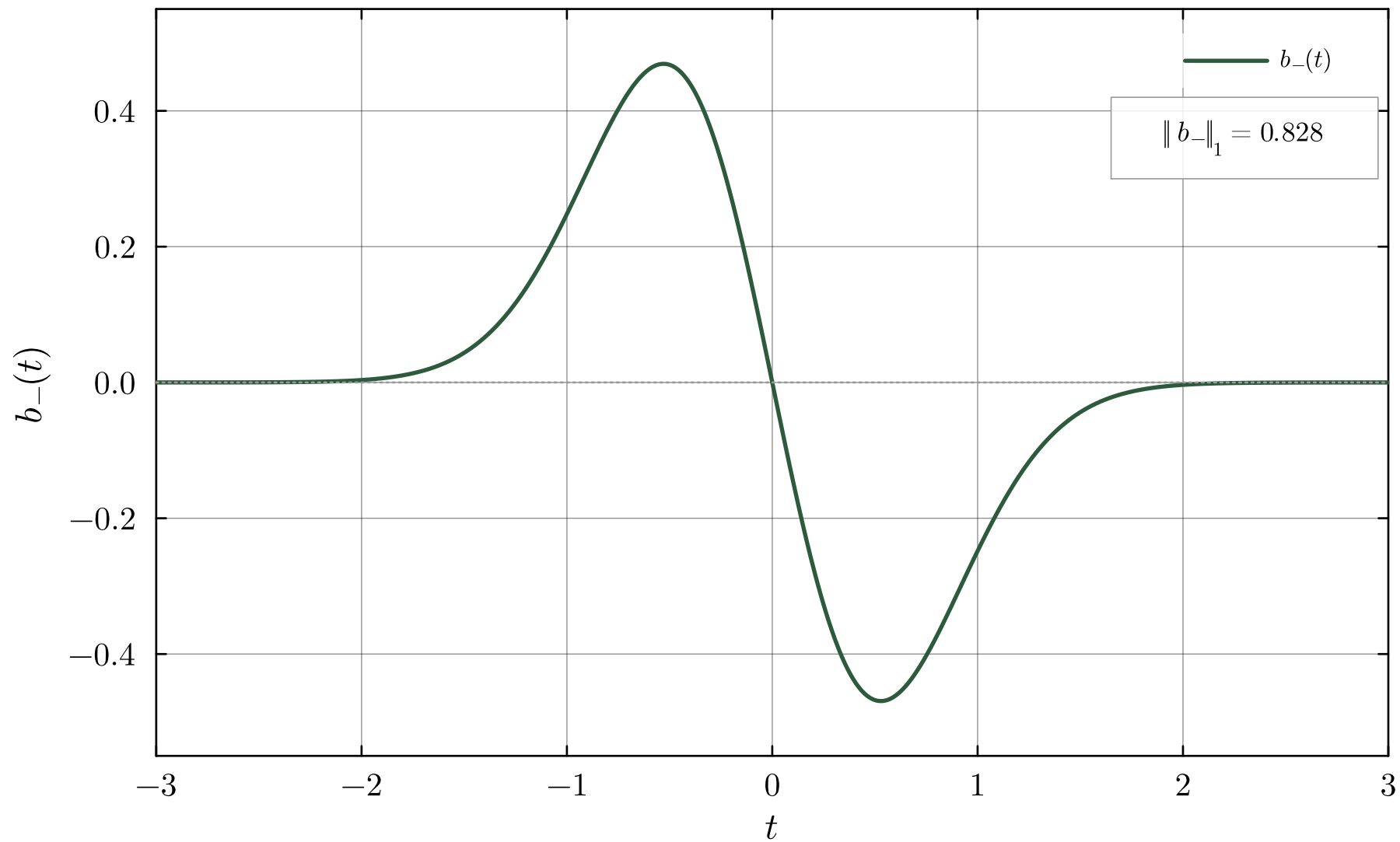
Outer kernel b_-(t) ( \bar{\beta} = 10 , \sigma = 1/\bar{\beta} )
