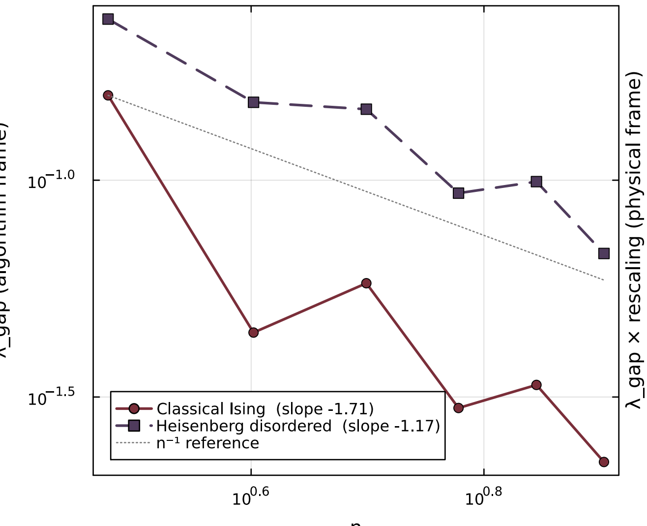
(a) gap_alg vs n ( \beta_{\text{phys}} = 0.5 )
