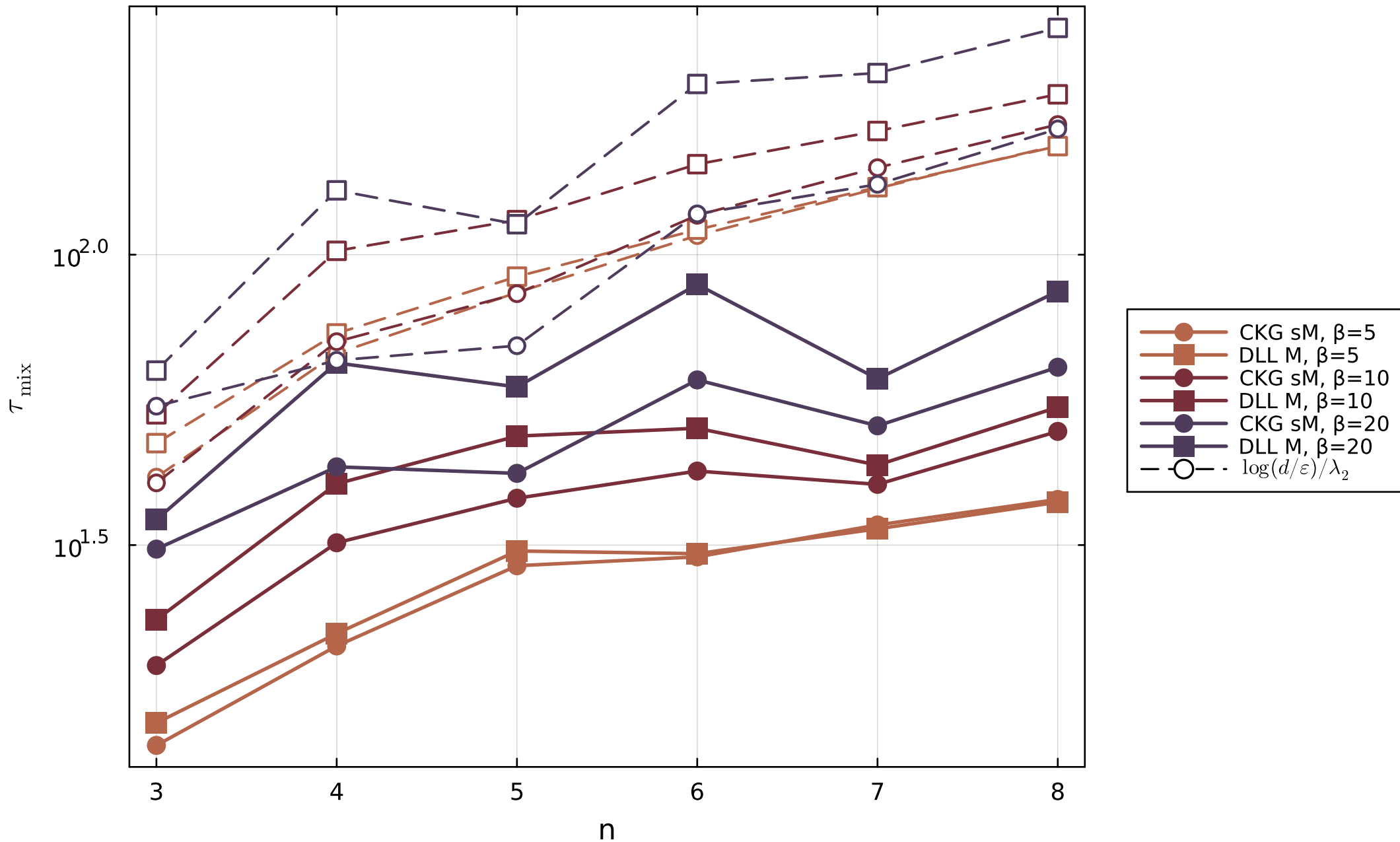
Ideal-Lindbladian \tau_{\text{mix}} \cdot 1\text{D XXX (zz-disorder)} \cdot \varepsilon = 1\text{e-}03
