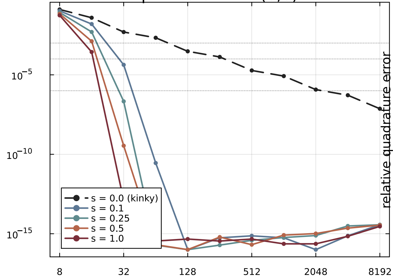
\beta = 10.0 - \nu=(0,0)
