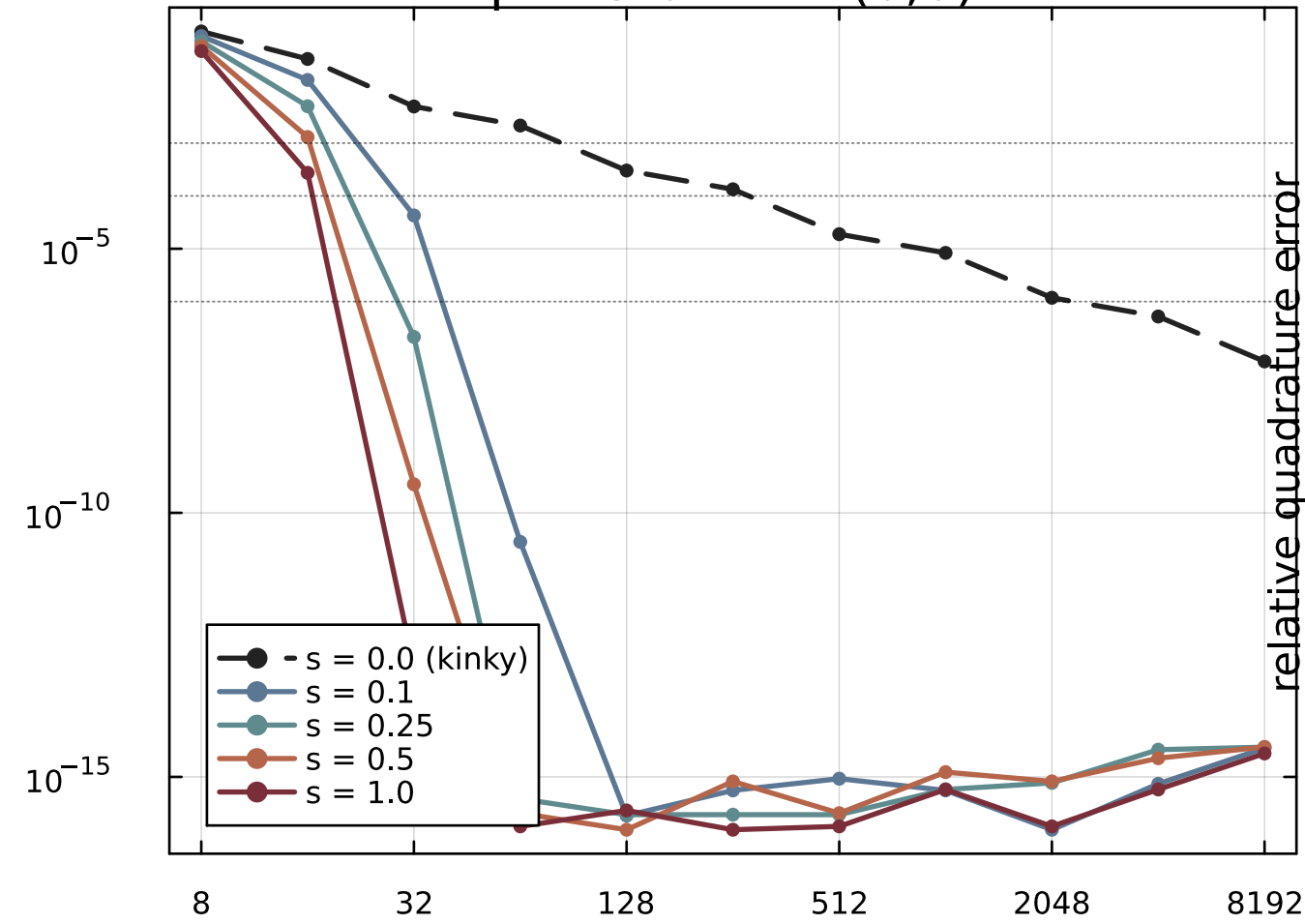
\beta = 5.0 - \nu=(0,0)
