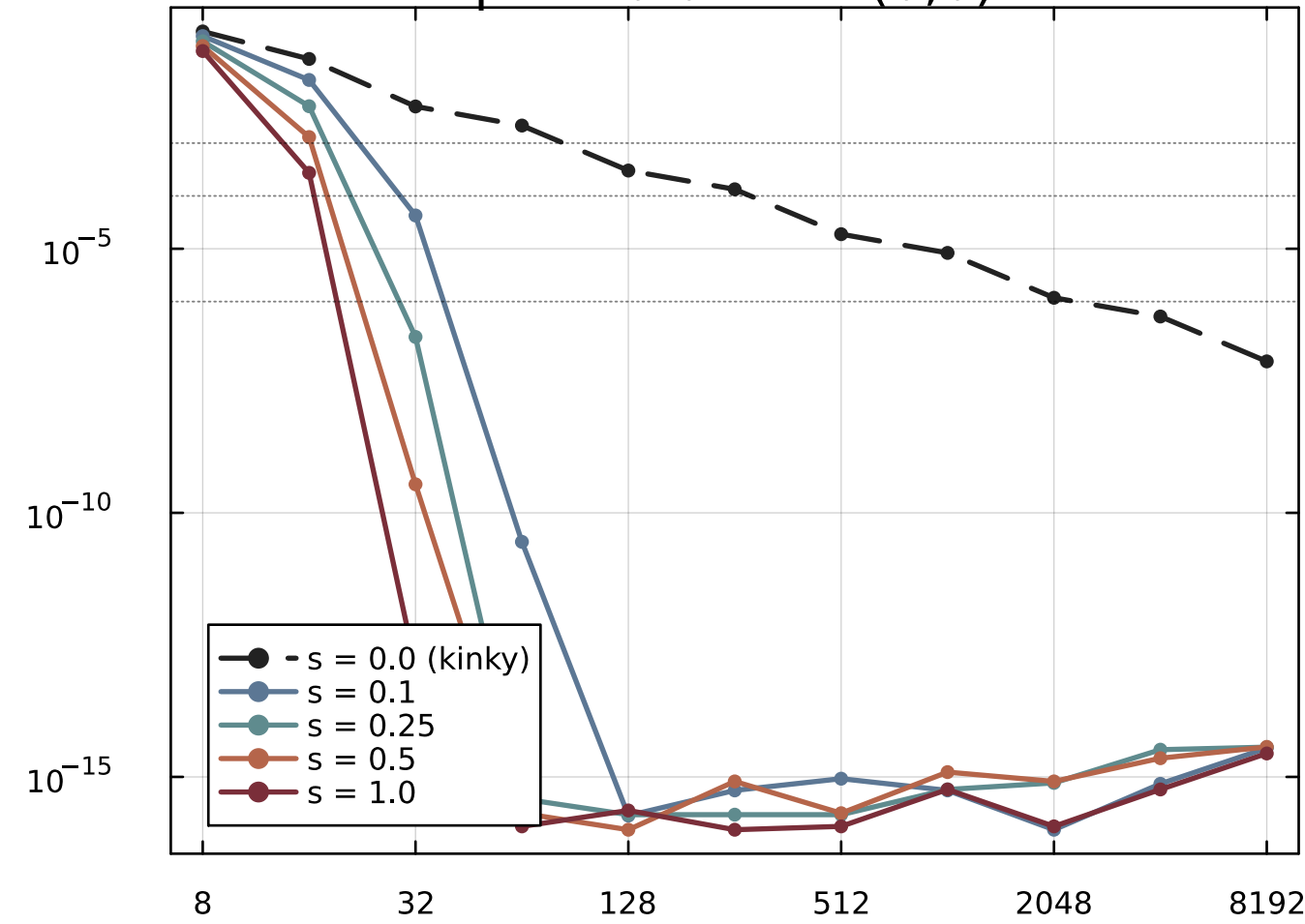
\beta = 20.0 - \nu=(0,0)
