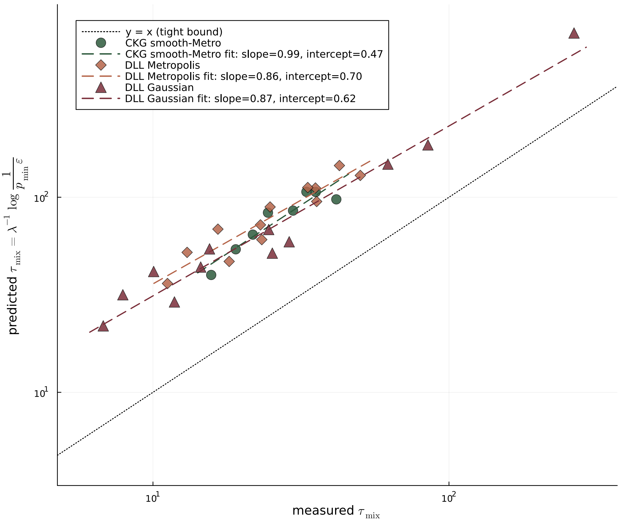
Spectral-gap bound vs measured \tau_{\text{mix}} (qf-mto.6)
