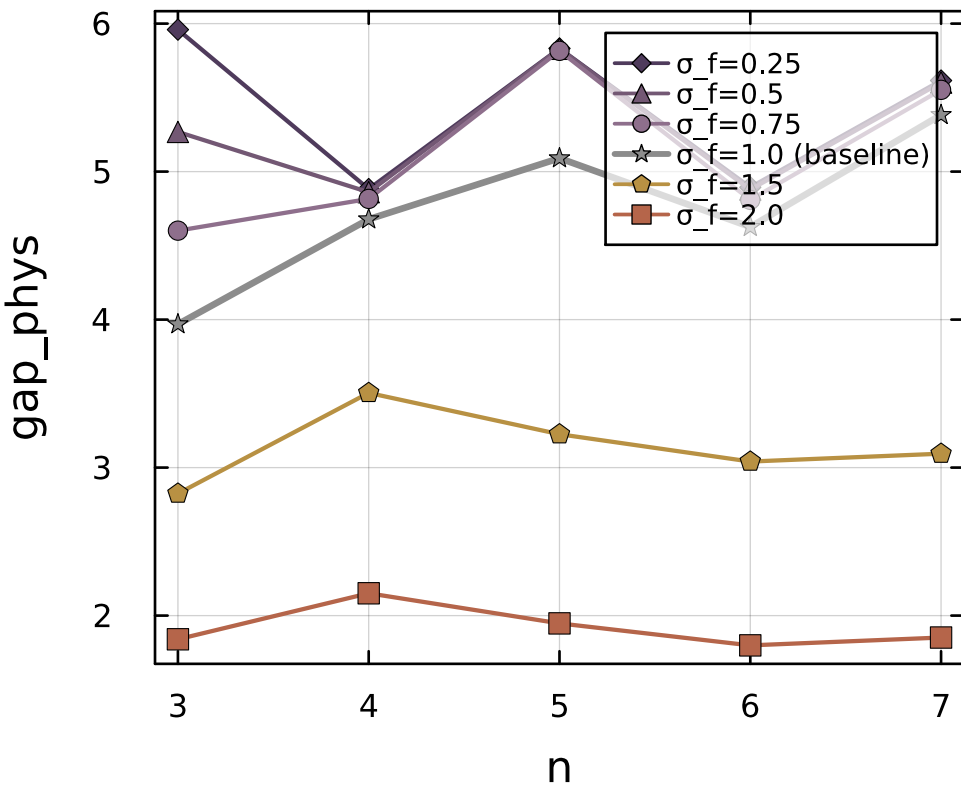
(a) Raw spectral gap ( \beta_{\text{phys}}=0.5 )
