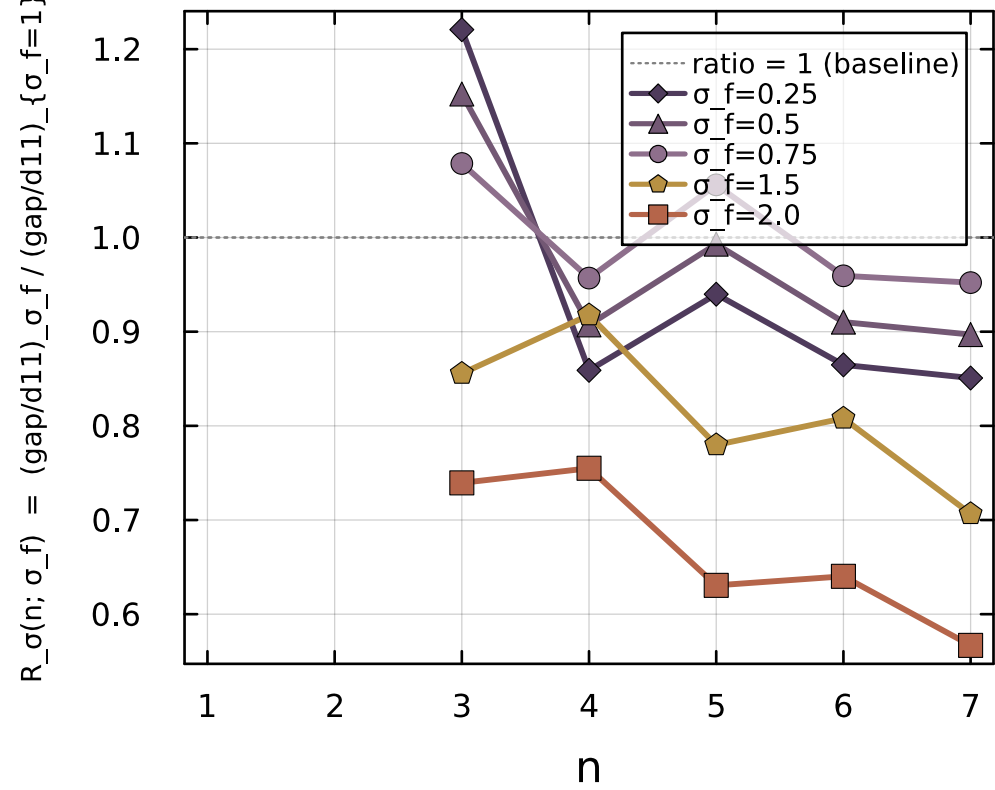
(c) \sigma -baseline ratio at \beta_{\text{phys}}=0.5
