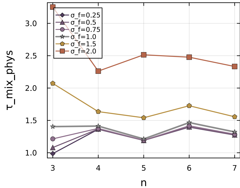
(b) Raw mixing time ( \beta_{\text{phys}}=0.5 )
