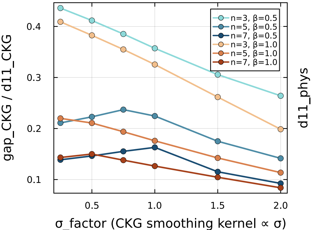
(a) \sigma -rate cancellation within CKG
