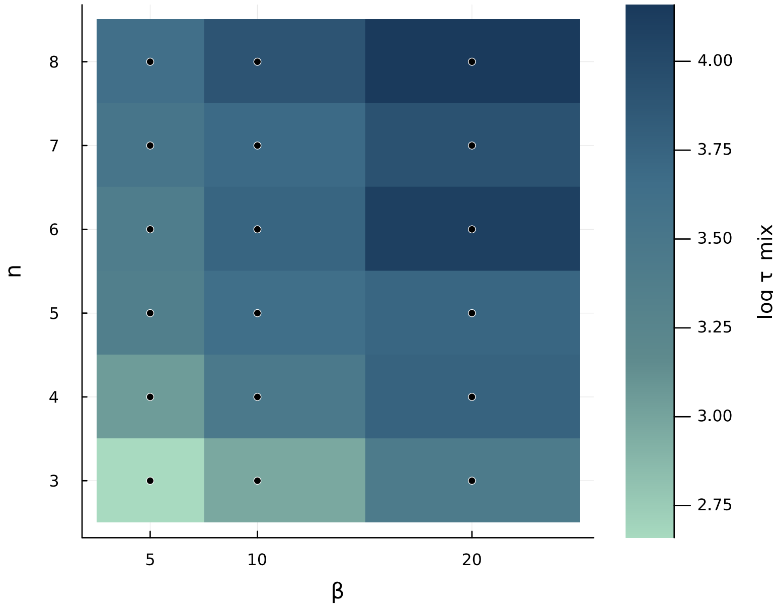
Observed \log \tau_{\text{mix}}
