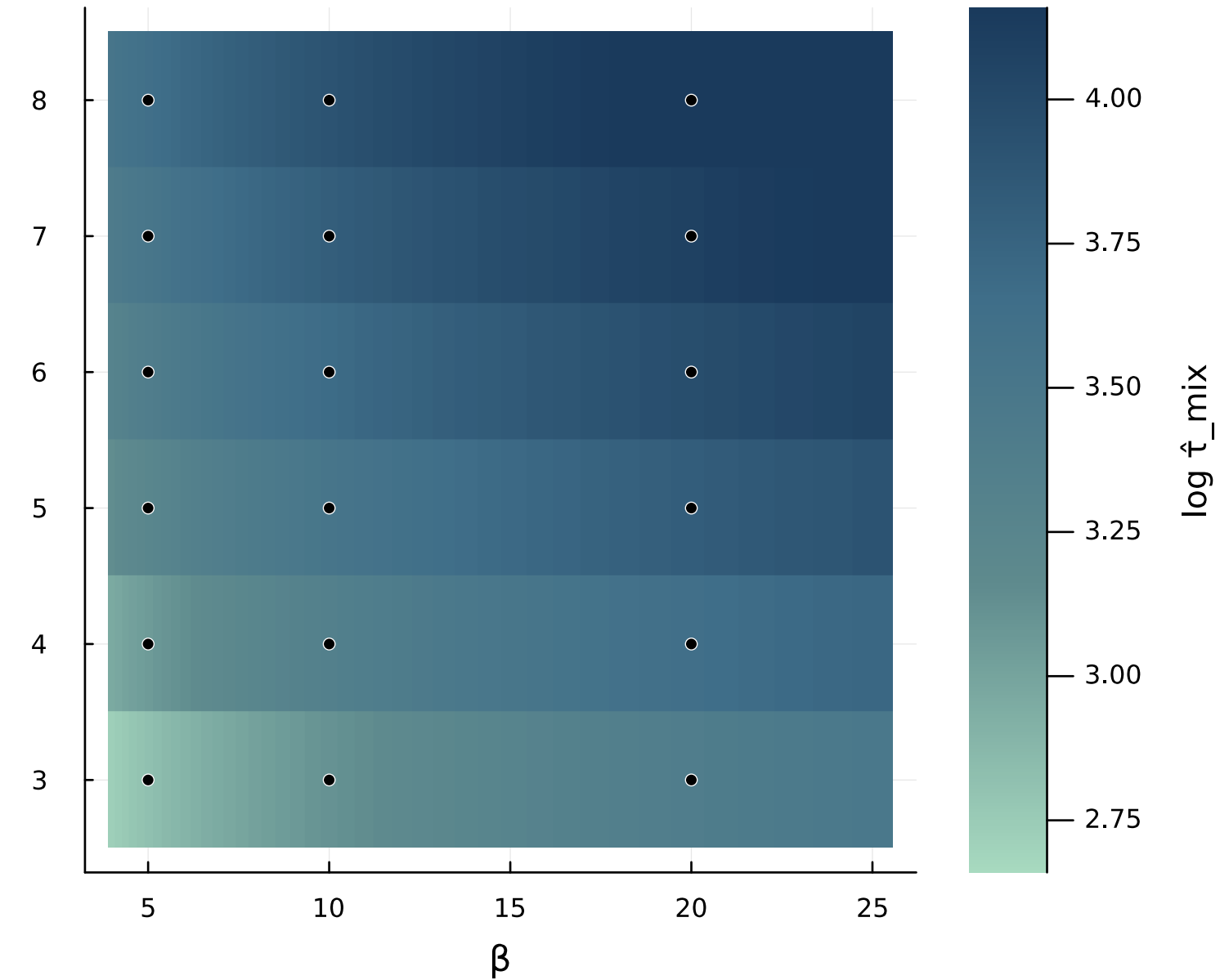
M0 fit \log \hat{\tau}_{\text{mix}}
