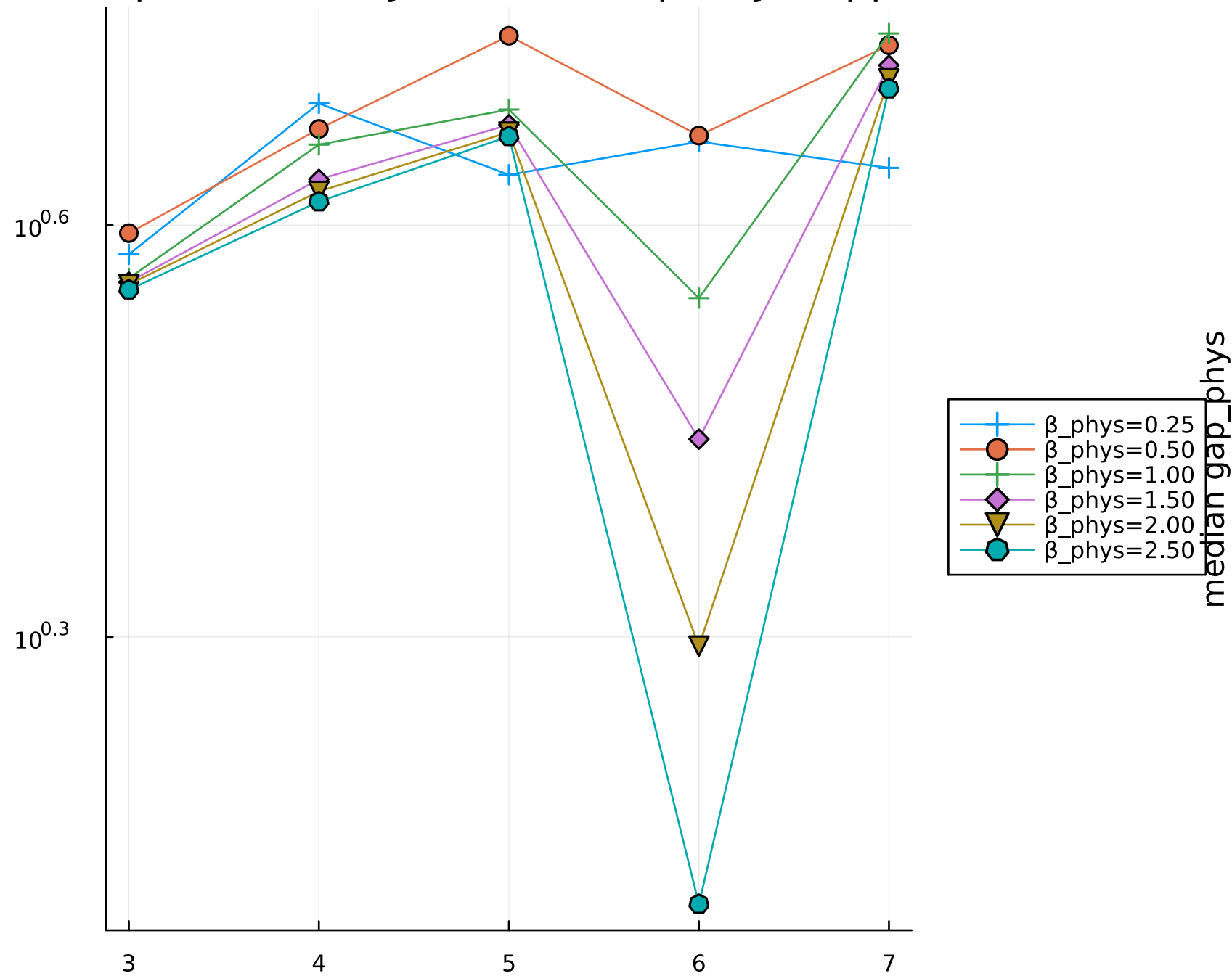
v6: \rho_0 = I/d + \text{krylovdim}=40 (parity-trapped)
