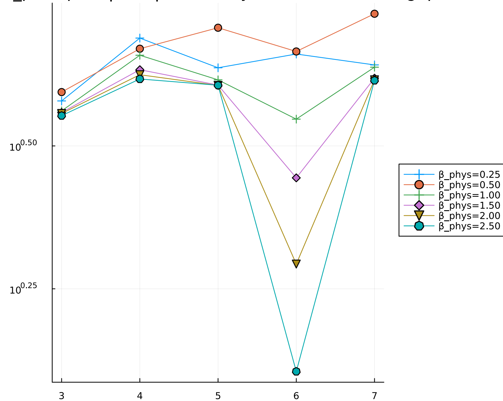
v6_plus: \rho_0 = |+\rangle\langle+|^{\otimes N} + \text{krylovdim}=60 (true L gap)
