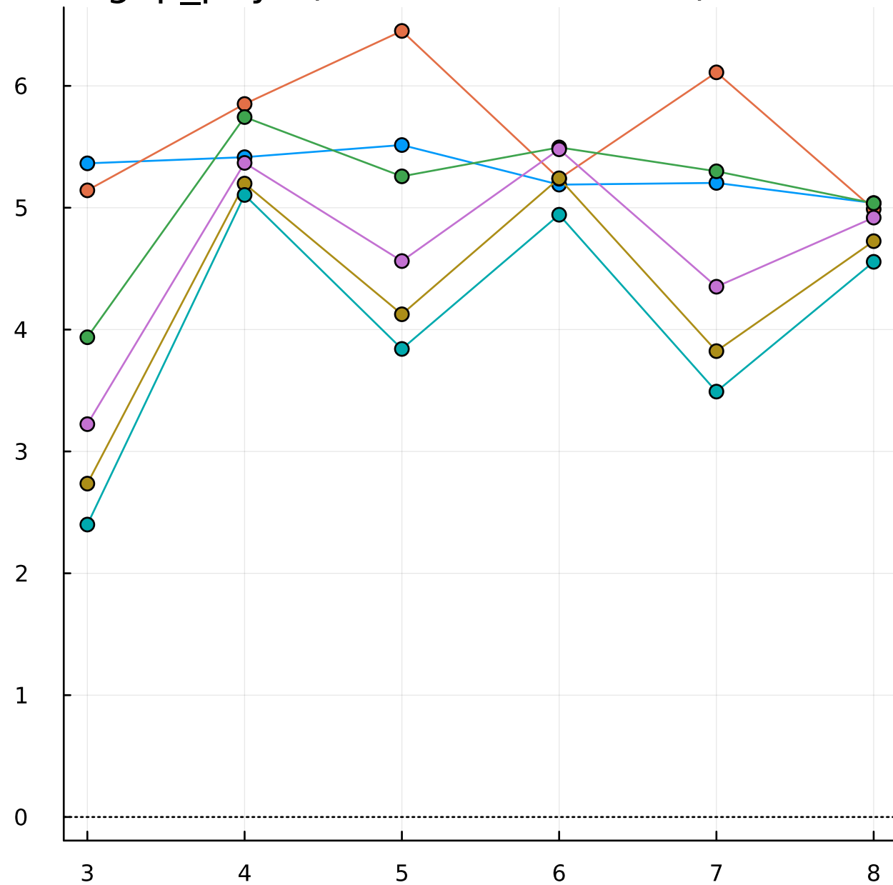
gap_phys (CKG smooth-Metro) — vs n
