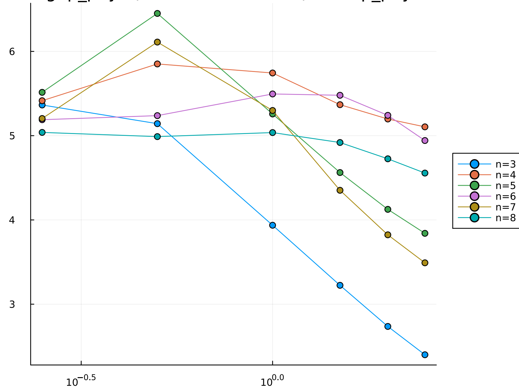
gap_phys (CKG smooth-Metro) — vs \beta_{\text{phys}}
