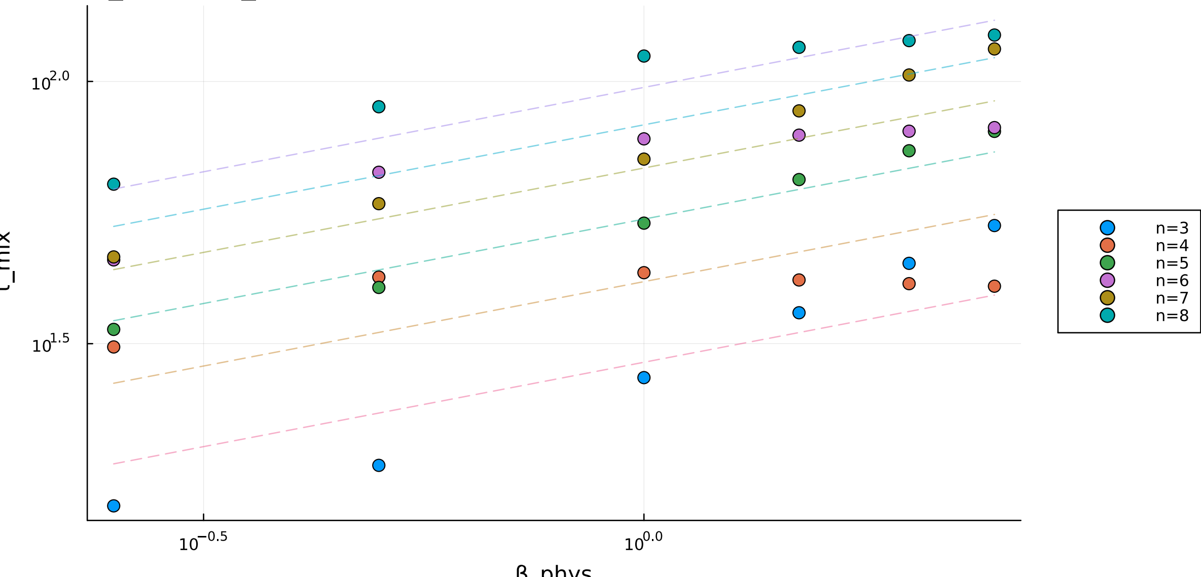
\tau_{\text{mix}} vs \beta_{\text{phys}} — 1D Heisenberg disordered, CKG smooth-Metro
