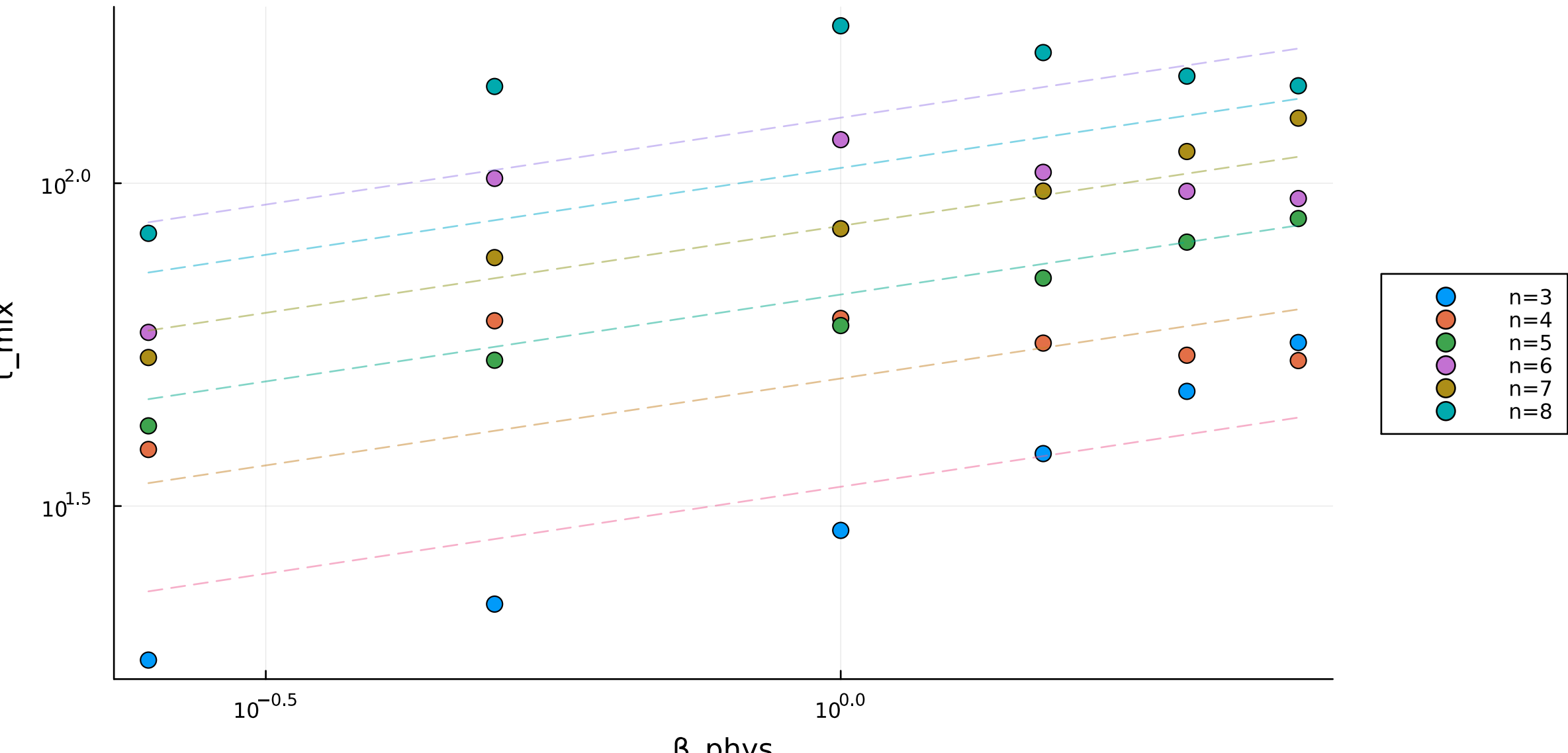
\tau_{\text{mix}} vs \beta_{\text{phys}} — 1D Heisenberg disordered, DLL Metropolis
