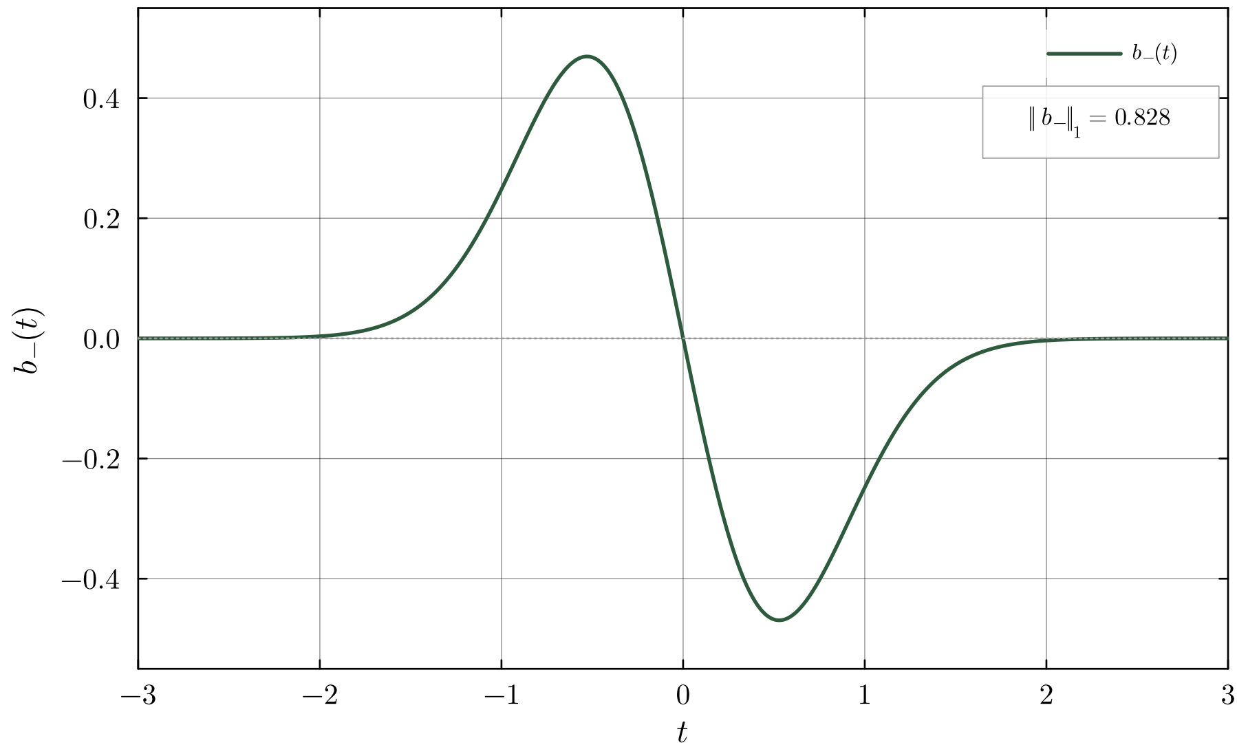
Outer kernel b_-(t) ( \beta = 10, \sigma = 1/\beta )
