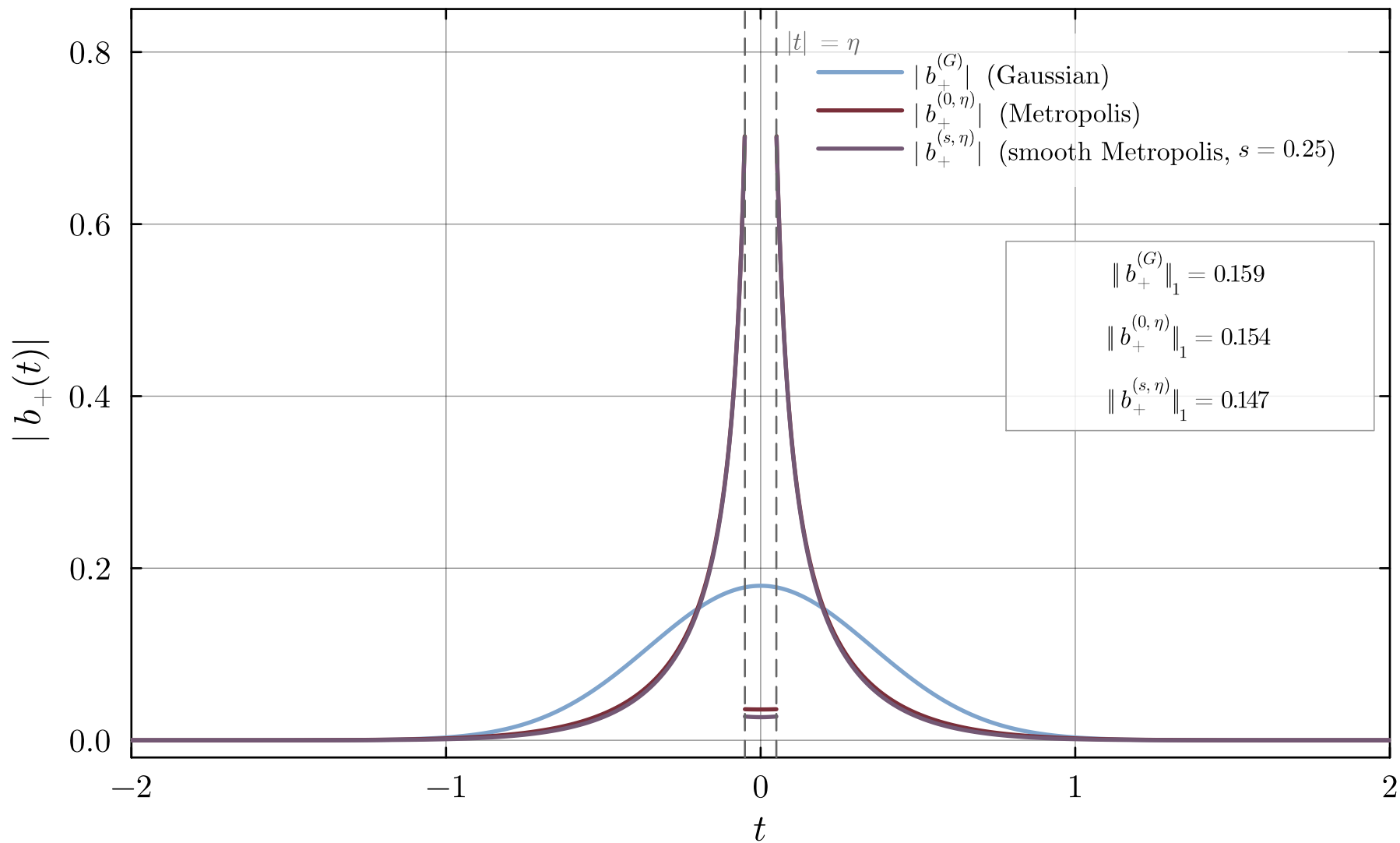
Coherent-term kernel |b_+(t)| ( \beta = 10 , \sigma = 1/\beta , \eta = 0.05 )
