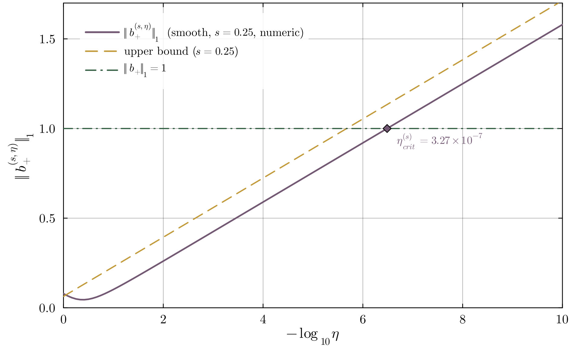
\ell_1 norm of the regularized Metropolis kernel ( \sigma = 1/\beta )
