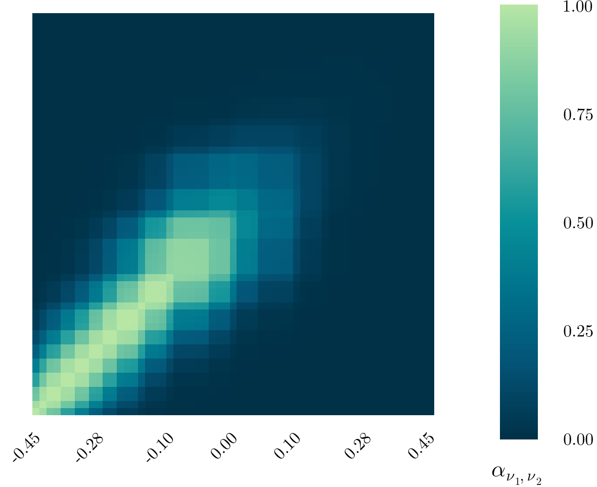
CKG (KMS DB), \beta = 20
