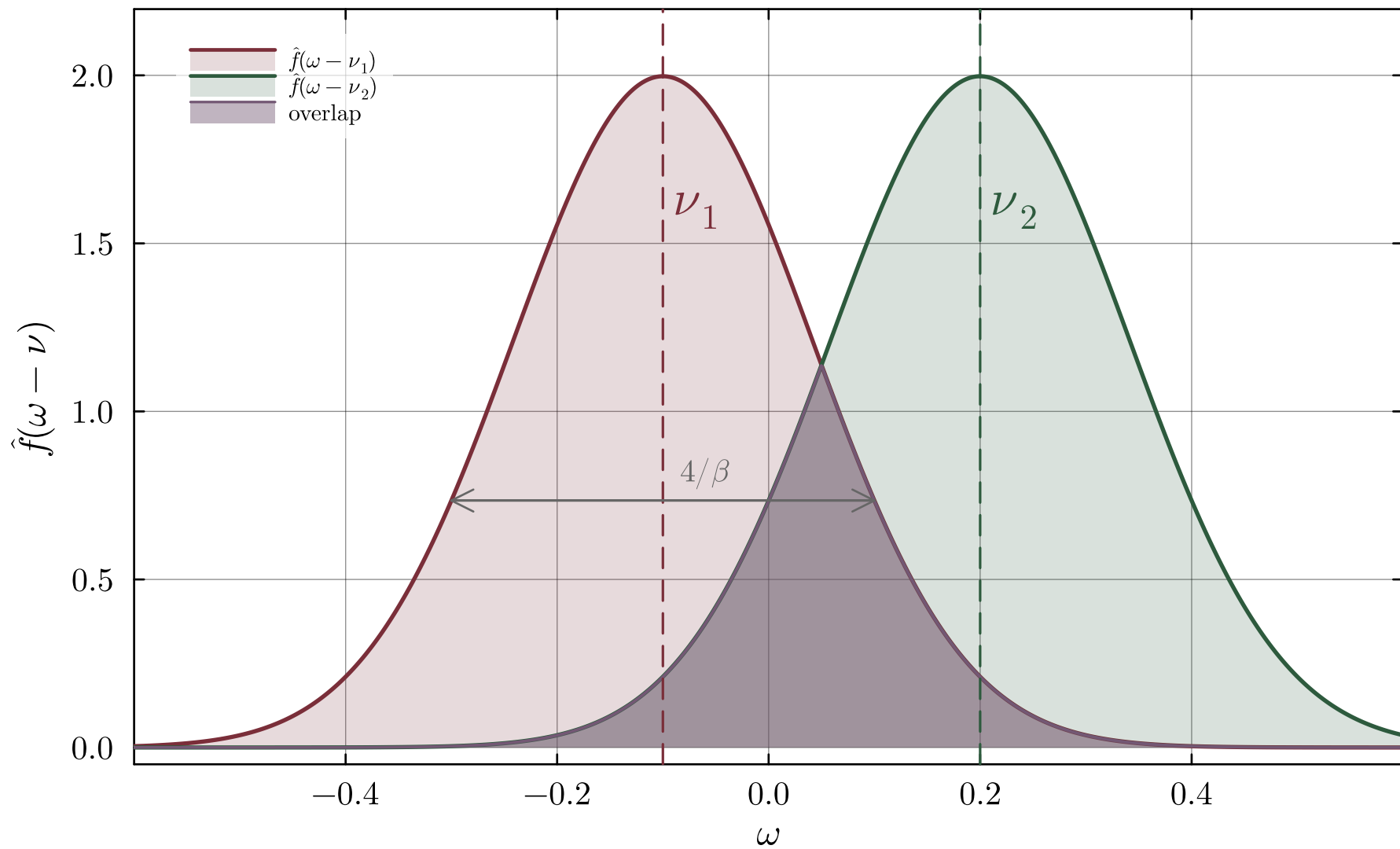
OFT Gaussian filtering around Bohr frequencies ( \beta = 10 , \sigma = 1/\beta )
