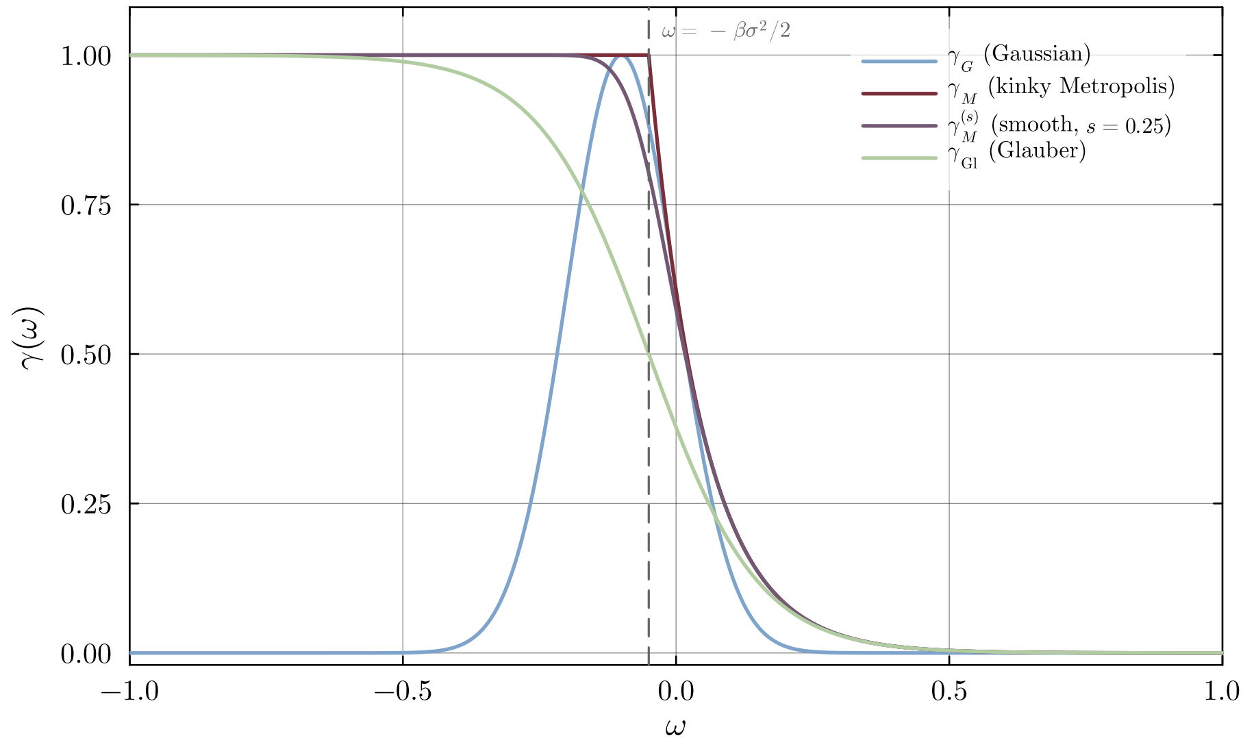
Transition weights ( \beta = 10 , \sigma = 1/\beta )
