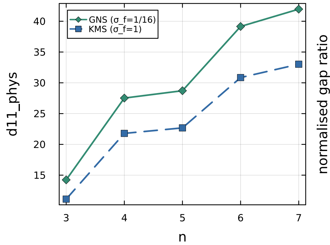
(b) d_{\{1 \rightarrow 1\}} vs n at each sampler's converged \sigma
