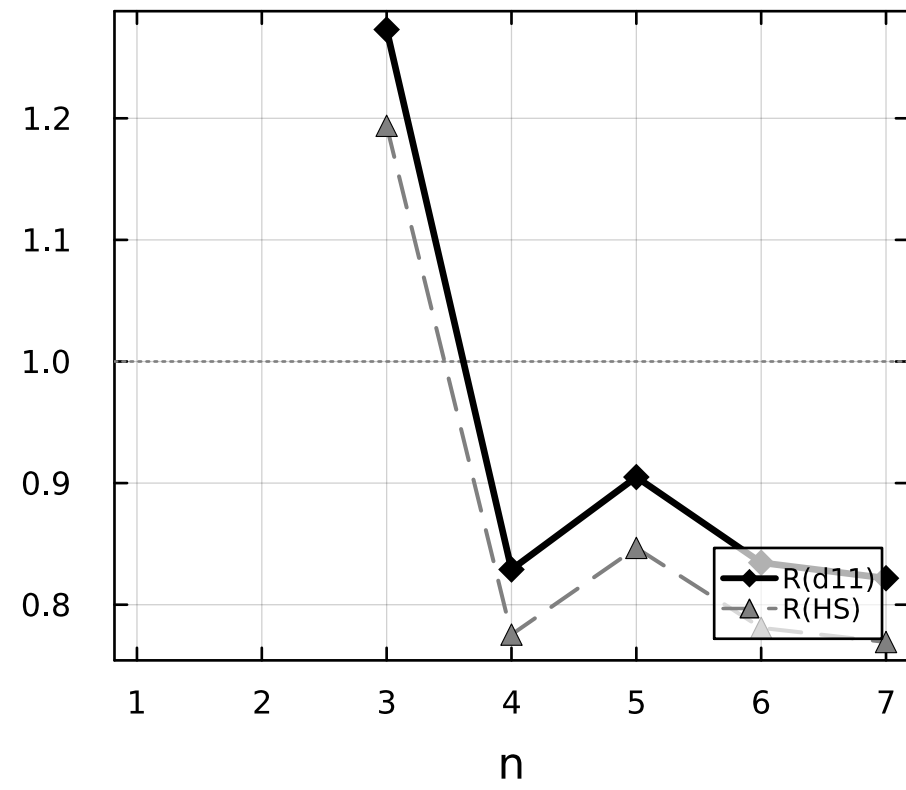
(c) Cross-norm at converged- \sigma cells
