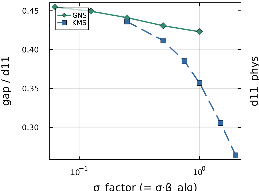
(a) \sigma -rate test within each sampler ( n=3 , \beta=0.5 )
